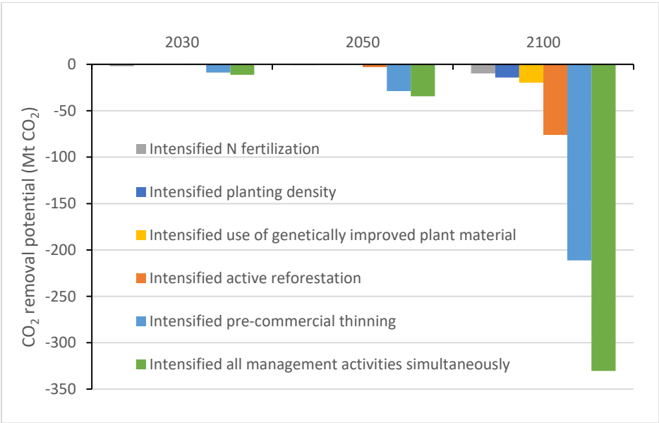
Figure 4. CO2 removal potential (Mt CO2) for selected forest management activities 2030 – 2100
