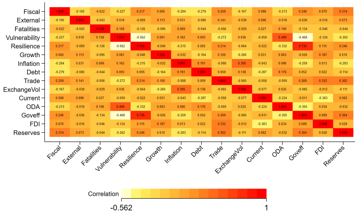
Figure 1: Correlation Map
