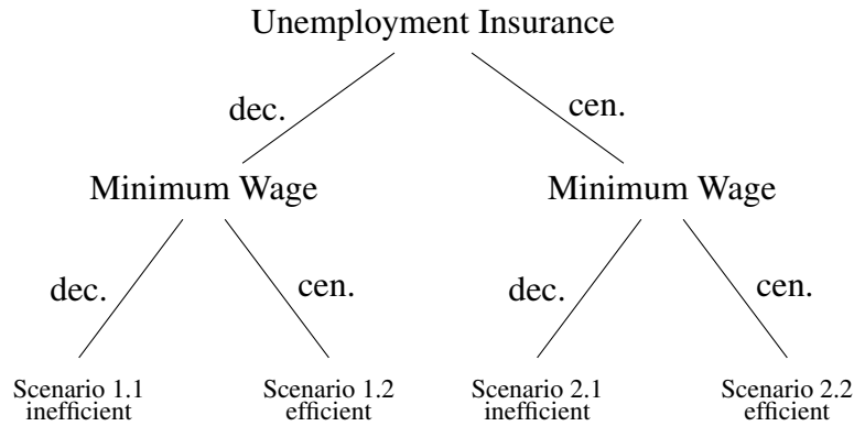
Figure 1: Results with symmetric states
