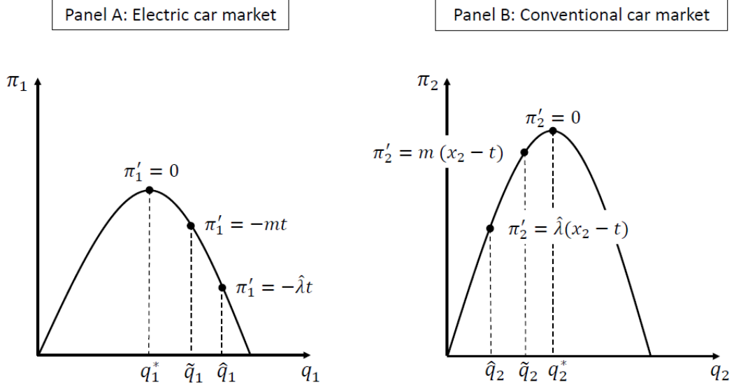
Figure 1: The figure shows the profit in the electric car market, \pi_1 := (p_1 - c_1)q_1 , in Panel A and the profit in the conventional car market, \pi_2 := (p_2 - c_2)q_2 , in Panel B. It illustrates part ii.b) of Proposition 1 when m < \hat{\lambda} holds and the VET solution (\tilde{q}_1, \tilde{q}_2) is optimal. In the electric car market (Panel A) the VET solution implies an output level, \tilde{q}_1 , above the benchmark solution, q_1^* , but below the FET solution, \hat{q}_1 . In the conventional car market (Panel B) the VET solution, \tilde{q}_2 , implies an output level above the FET solution, \hat{q}_2 , but still below the benchmark level, q_2^* .
