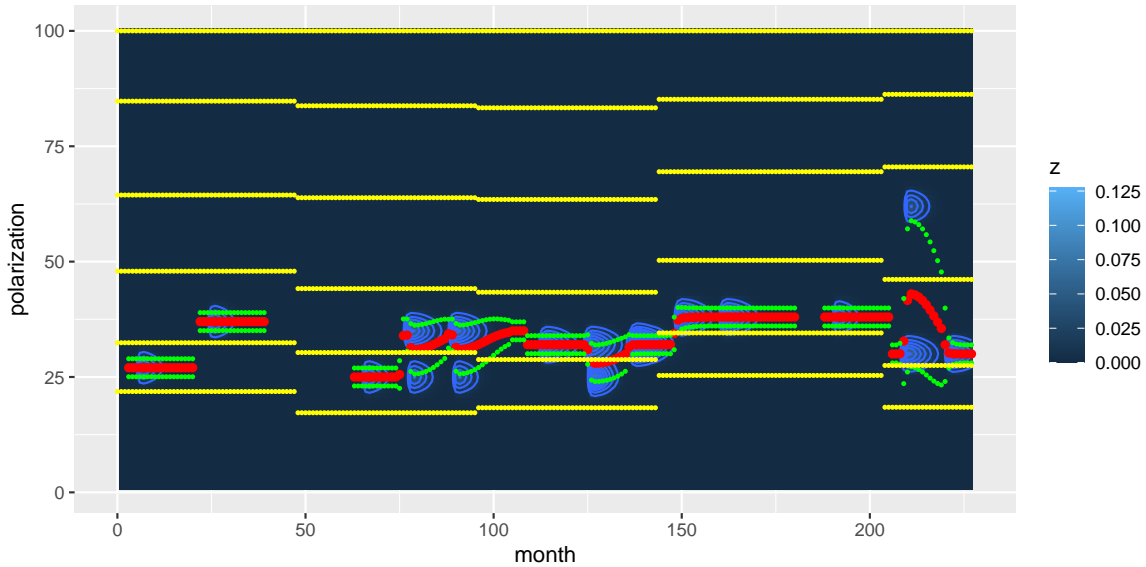
Figure A.3: Political classification using endorsements, party events and think tanks
