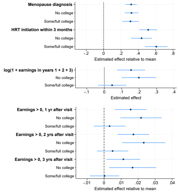
(c) Baseline, with 30 day donut and controlling for prior earnings
