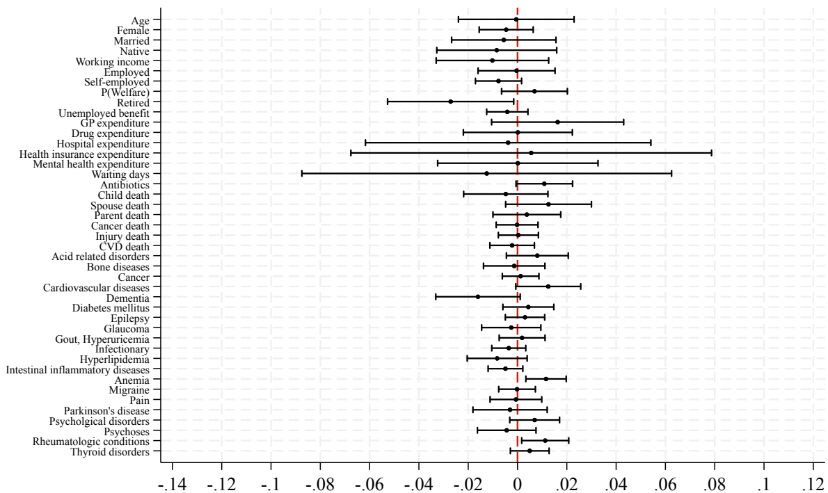
Figure 4: Balancing test
