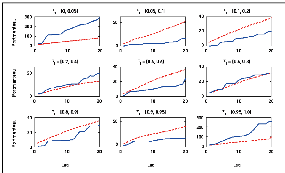
Box-Ljung test statistic \hat{Q}_\tau^{(p)} for each lag p using \hat{\beta}_\tau(k) . Same as Figure 4(b).
