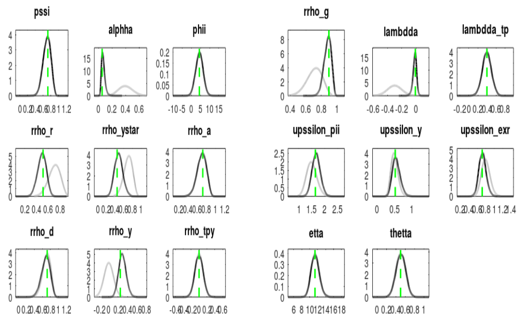
Figure 3: Prior-Posterior Plots
