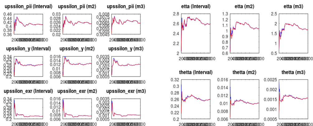
Figure 5: MCMC Univariate Diagnostics for selected parameters
