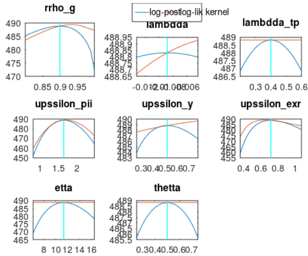
Figure 4: Mode Check Plot
