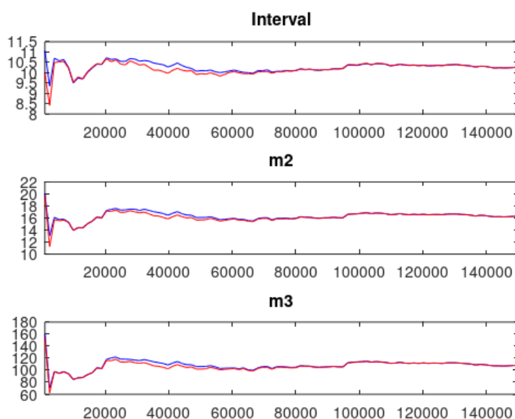
Figure 6: Multivariate Convergence Diagnostic
