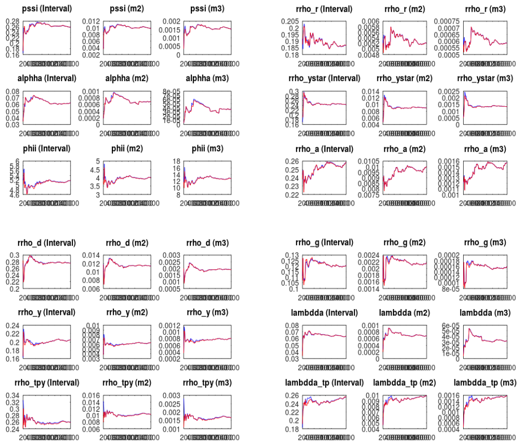
Figure 4: Mode Check Plot
