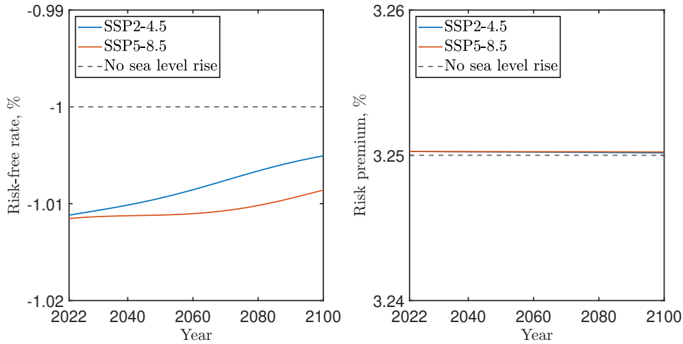
Figure 9: Optimal risk-free rate and risk premium under the SSP2-4.5 and SSP5-8.5 scenarios, compared to a scenario with no sea level rise.
