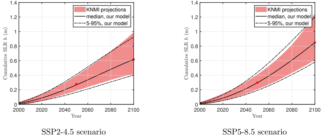
Figure 2: Comparison between our model (9) and KNMI projections for cumulative sea level rise and its distribution along the Dutch North Sea coast for the SSP2-4.5 and SSP5-8.5 scenarios. The shaded red area shows the 5-95% confidence band from Van Dorland et al. (2023). The lines in the figure are the fitted 5th, 50th, and 95th percentiles of our model. Red dots indicate the median of the KNMI projection for sea level rise, which is given for 2050 and 2100.
