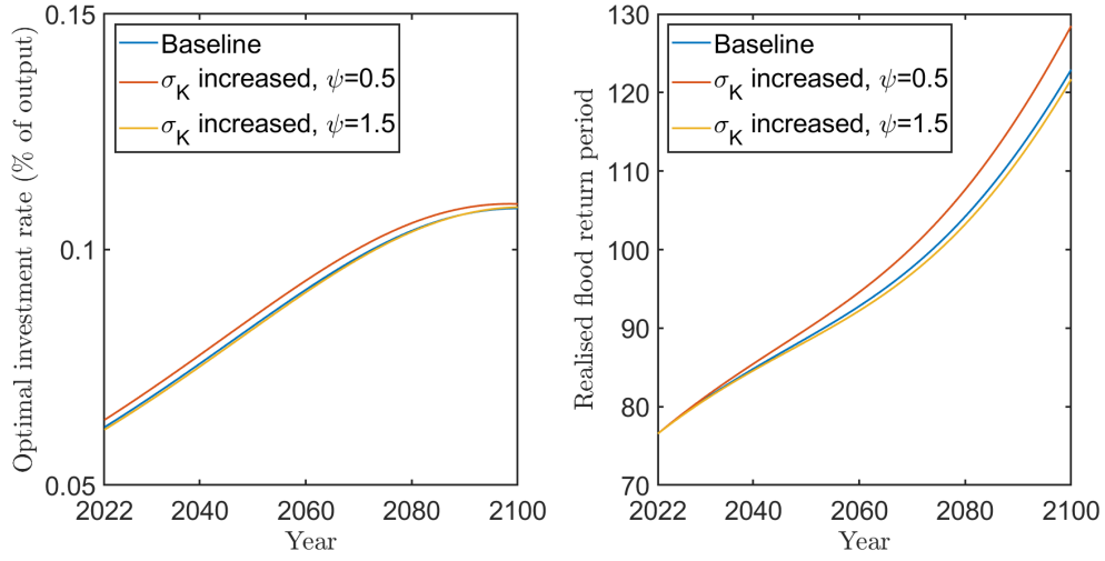
Figure 11: Effects of higher macroeconomic volatility \sigma_K on optimal flood protection investment and the return period under the SSP5-8.5 scenario without sea level rise uncertainty. The volatility is increased by 44%.
