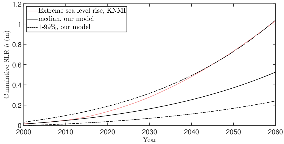
Figure 13: The red line is projected sea level rise given abrupt collapse of the Arctic Ice Sheet provided by KNMI. The solid black line is the fitted median, and the dotted lines are the 1st and 99th percentiles of the fitted process.
