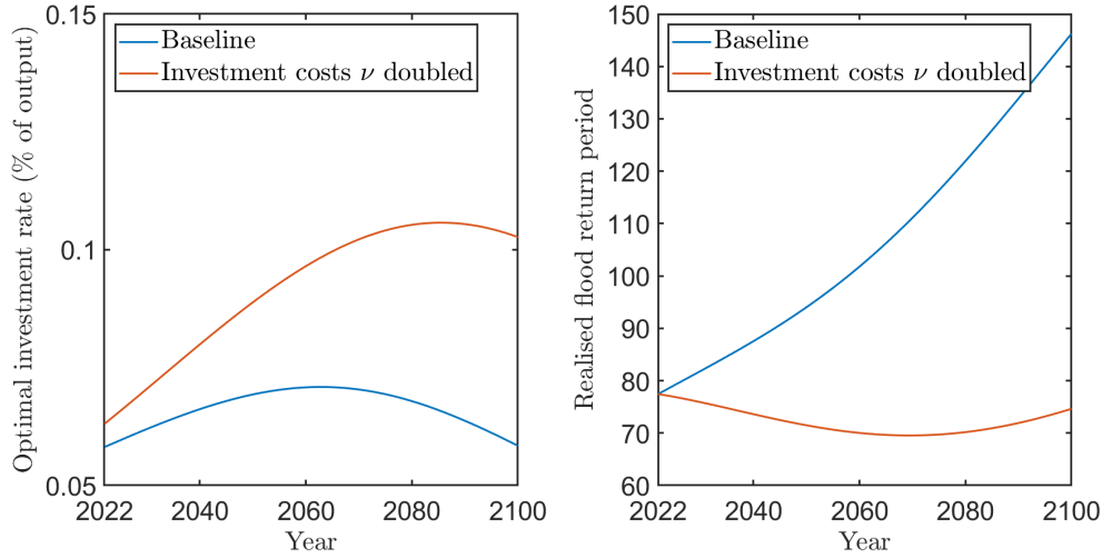
Figure 7: Effects of doubling investment costs on optimal flood protection investment and return period under the SSP2-4.5 scenario with no sea level rise uncertainty. Relative to the baseline, the cost parameter \nu is doubled while the adjustment cost parameter \theta_H is halved. This way, investment capacity is unaffected (adjustment costs stay constant given dyke heightening).
