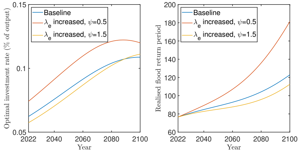
Figure 12: Effects of a higher risk of macroeconomic disasters on optimal flood protection investment and the return period under the SSP5-8.5 scenario without sea level rise uncertainty. The disaster arrival rate is increased by 44%, so that the discount rate falls to 1%.
