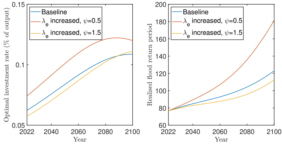
Figure 12: Effects of a higher risk of macroeconomic disasters on optimal flood protection investment and the return period under the SSP5-8.5 scenario without sea level rise uncertainty. The disaster arrival rate is increased by 44%, so that the discount rate falls to 1%.
