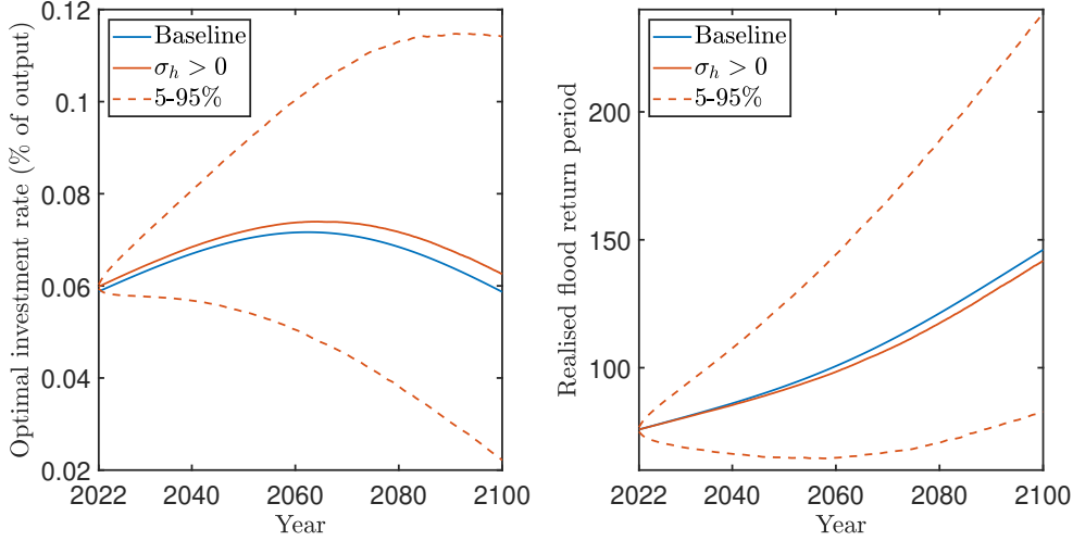
Figure 5: Effects of stochastic sea level rise on optimal flood protection investment and the return period under the SSP2-4.5 scenario. The blue line shows the deterministic path; the red line shows the mean of the stochastic path; and the dashed lines show the 5 and 95 percentiles of the stochastic paths. In the right panel, the red line shows the inverse of the mean flood arrival rate.
