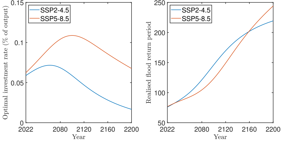
Figure 3: Optimal flood protection investment and the return period of flooding for the global warming scenarios SSP2-4.5 and SSP5-8.5 without sea level rise uncertainty (baseline results).
