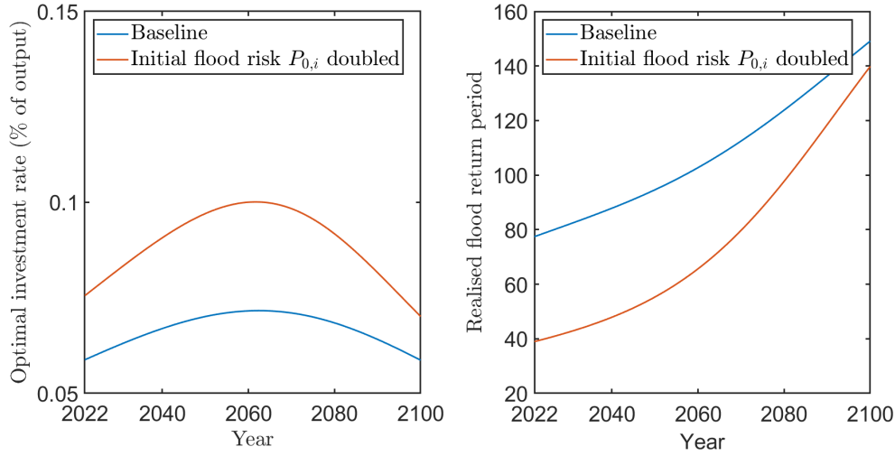
Figure 6: Effects of doubling the initial flood arrival rate, P_{0,i} in each zone on optimal flood protection investment and the return period under the SSP2-4.5 scenario with no sea level rise uncertainty.
