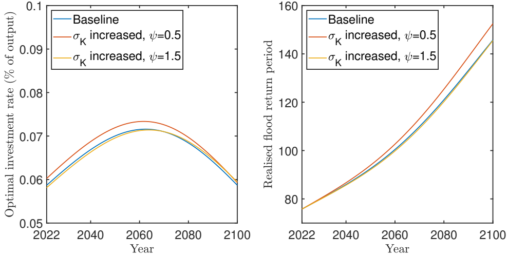
Figure 10: Effects of higher macroeconomic volatility \sigma_K on optimal flood protection investment and the return period under the SSP2-4.5 scenario without sea level rise uncertainty. The volatility is increased by 44%.
