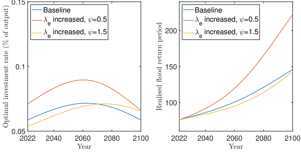
Figure 4: Effects of a higher risk of macroeconomic disasters on optimal flood protection investment and the return period under the SSP2-4.5 scenario without sea level rise uncertainty. The disaster arrival rate is increased by 44%, so the discount rate falls to 1% for \psi = 0.5 .
