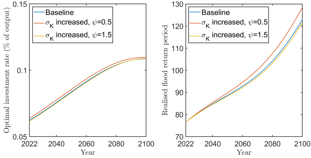
Figure 11: Effects of higher macroeconomic volatility \sigma_K on optimal flood protection investment and the return period under the SSP5-8.5 scenario without sea level rise uncertainty. The volatility is increased by 44%.
