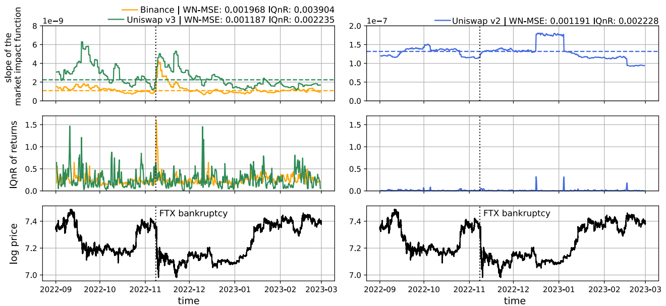
Fig. 4 Slope of market impact function for order book event resolved data with median lines (first row), IQnR of returns (second row) and log-price evolution (third row) for the ETH/USD pair on Binance (left, orange), Uniswap v3 (left, green) and Uniswap v2 (right, blue) for a rolling window width \Delta T = 1d over the analysis period 2022-09-01 to 2023-02-28 \Delta T = 6M
