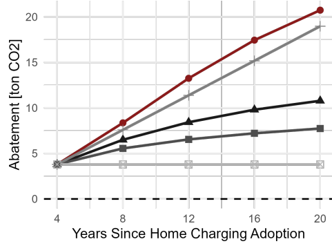
(a) Cumulative Emissions Abatement
