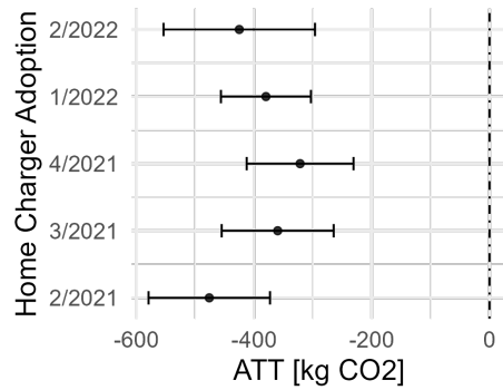
(c) CO 2 Emissions (EU ETS Cap)
