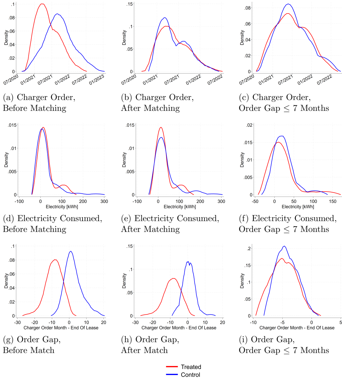
Figure E.7: Kernel Density Plots Before and After Matching
