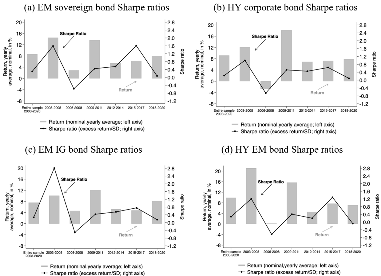
Figure 6. Sharpe ratios
