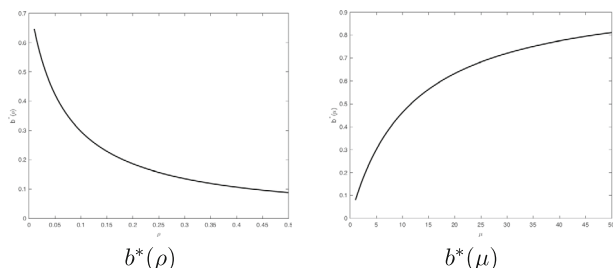
Fig. 4 Dependency of b^* with respect to \rho and \mu
