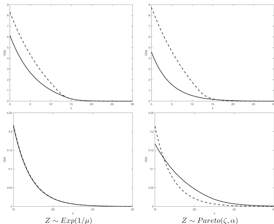
Fig. 8 Value function (zoomed image in the bottom panels) in the case of proportional reinsurance (solid line) and excess-of-loss reinsurance (dashed line), when the claim sizes Z \sim \text{Exp}(1/\mu) (left panel) and Z \sim \text{Pareto}(\zeta, \alpha) (right panel)
