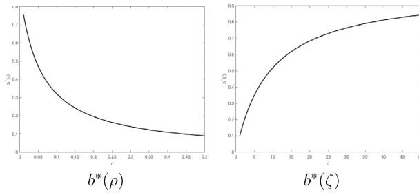
Fig. 6 Dependency of b^* with respect to \rho and \zeta
