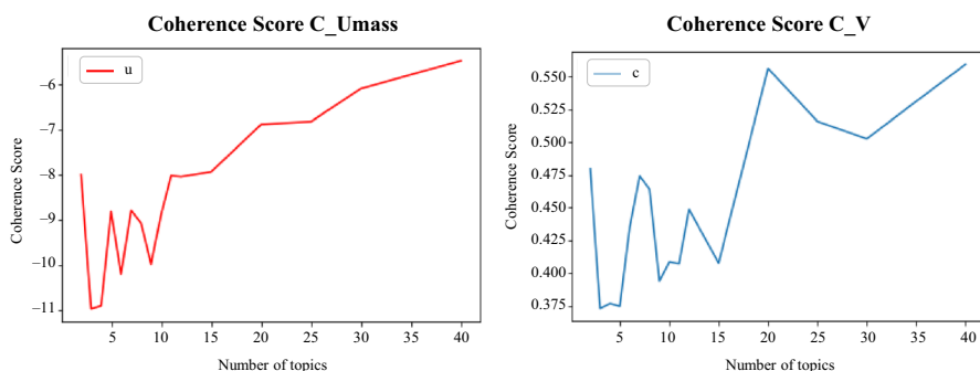
Fig. 5 Comparison of the topic model coherence scores C\_Umass and C\_V
