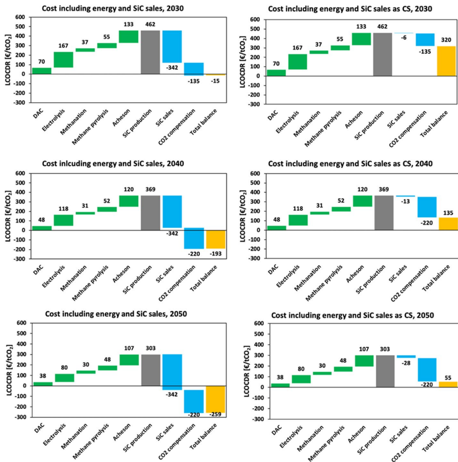
Fig. 4 LCODR of e-SiC production with energy cost including SiC sales (left) and to substitute construction sand (right) and CO 2 pricing for 2030, 2040 and 2050. Abbreviation: CS, construction sand
