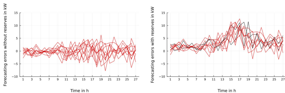
Fig. 16 Forecasting errors of solar PV generation and electricity demand without any planned reserves (left) and with planned reserves (right) in the ICC model
