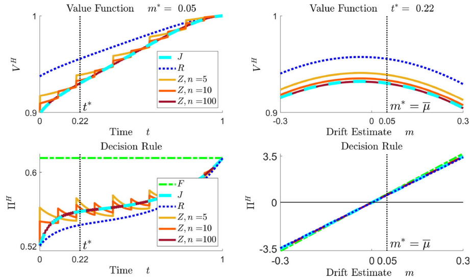
Fig. 4 Asymptotic behavior of value functions and optimal decisions rules for growing n and \Gamma(n) = \frac{n}{T} \sigma_J^2 . Top: Value functions V^H(t, m) depending on t/m (left/right) for H = R, J, Z Bottom: Optimal decision rules \Pi^H(t, m) for H = F, R, J, Z depending on t/m (left/right)
