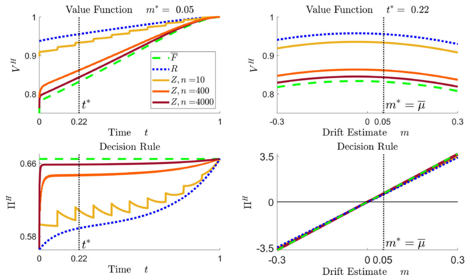
Fig. 5 Asymptotic behavior of value functions and optimal decision rules for growing n and \Gamma = 0.4 (fixed). Top: Value function \bar{V}^F(t, m, Q_t^{Z, 4000}) and V^H(t, m) depending on t/m (left/right) for H = R, Z . Bottom: Optimal decision rules \Pi^H(t, m) for H = F, R, Z depending on t/m (left/rights)
