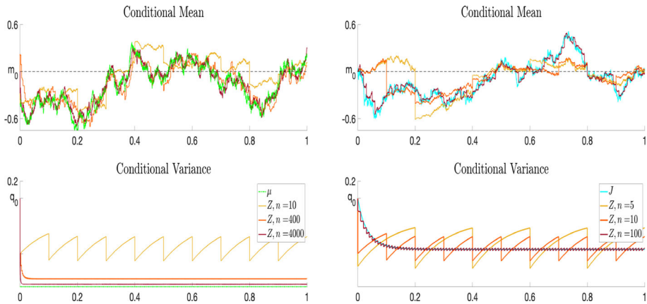
Fig. 2 Asymptotic behavior of the filter for n \rightarrow \infty Left: Constant expert's variance \Gamma = 0.4 , convergence to full information Right: Linearly growing expert's variance \Gamma^{(n)} = \frac{\eta}{T} \sigma_J^2 , diffusion approximation
