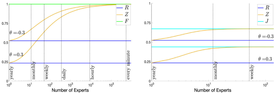
Fig. 6 Efficiency of the Z -investor for increasing n and power utility function with \theta = \pm 0.3 : Left: Expert's variance \Gamma = 0.4 fixed; Right: Expert's variance \Gamma^{(n)} = \frac{n}{7} \sigma_J^2 linearly growing
