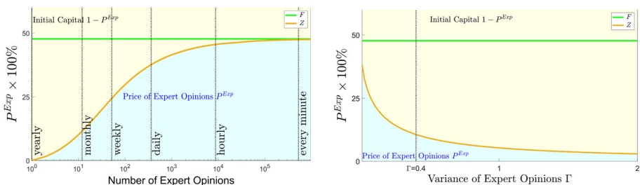
Fig. 7 Price of the experts for power utility with \theta = -0.3 : Left: Increasing number n of expert opinions and expert's variance \Gamma = 0.4 fixed; Right: Increasing expert's variance \Gamma and n = 10 fixed
