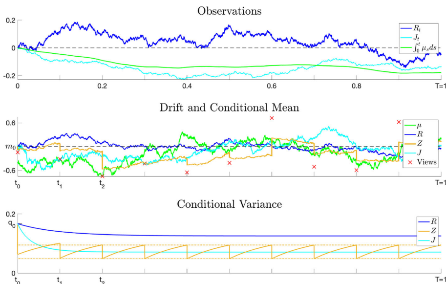
Fig. 1 Observation and filter processes. Top: Diffusion-type observation processes \mathbb{R} and J . Middle: Drift \mu , expert views Z_k and conditional mean M^H for H = R, Z, J . Bottom: Conditional variance Q^H
