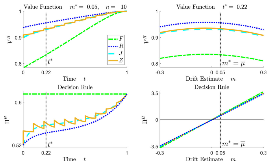
Fig. 3 Value functions and optimal decision rules. Top: Value functions V^H(t, m) for H = F, R, J, Z ( n = 10 ) depending on t/m (left/right). Bottom: Optimal decision rule \Pi^H(t, m) depending on t/m (left/right)
