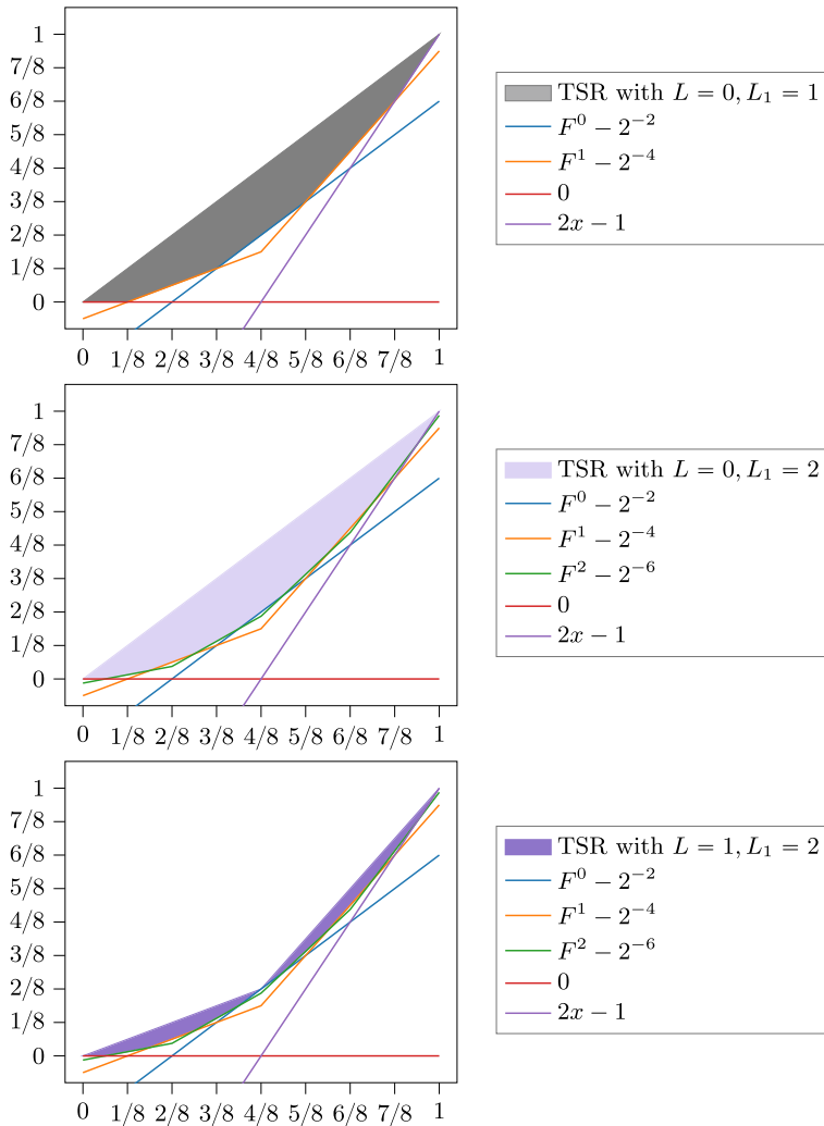
Fig. 4 The tightened sawtooth relaxations R^{L,L_1} from Definition 7 for the pairs (L, L_1) = (0, 1), (0, 2), (1, 2) . By increasing L_1 beyond L , we tighten the lower bound by creating more inequalities. This is done by only adding linearly-many variables and inequalities in the extended formulation to gain exponentially-many equally spaced cuts in the projection
