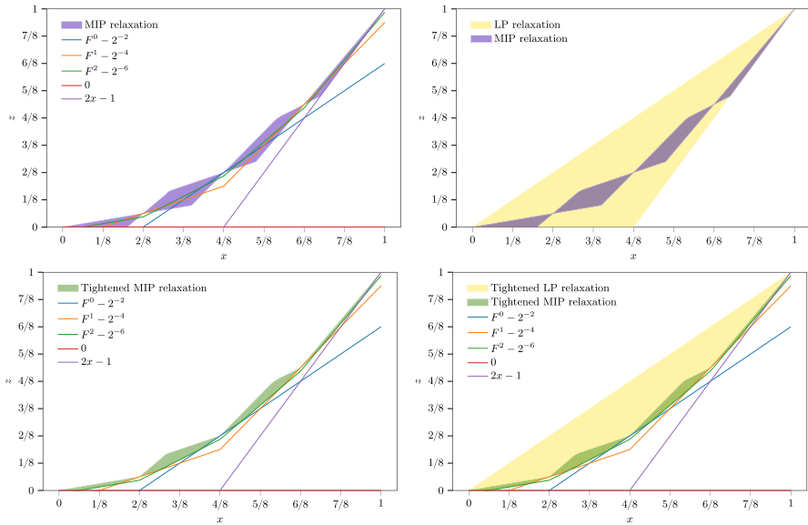
Fig. 3 Feasible set of the univariate MIP relaxation NMDT and its LP relaxation with L = 2 . In three of the plots we display the lower bounds obtained from tightening to show how this affects the MIP relaxation
