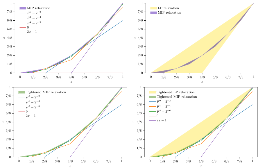
Fig. 2 Feasible set of the univariate MIP relaxation D-NMDT and its LP relaxation with L = 2 . In three of the plots, we display the lower bounds obtained from tightening to show how this affects the MIP relaxation
