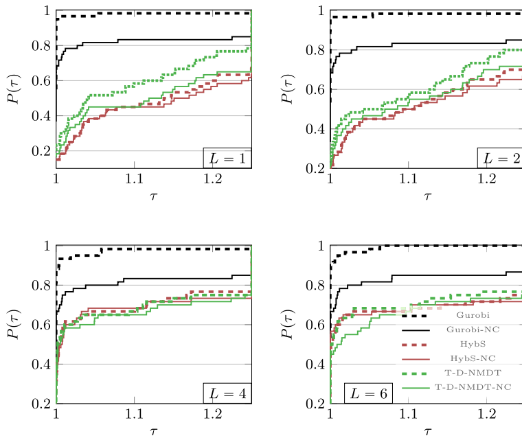
Fig. 7 Performance profiles on dual bounds of best MIP relaxation compared to Gurobi as MIQCQP solver, with and without cuts, on all 60 instances
