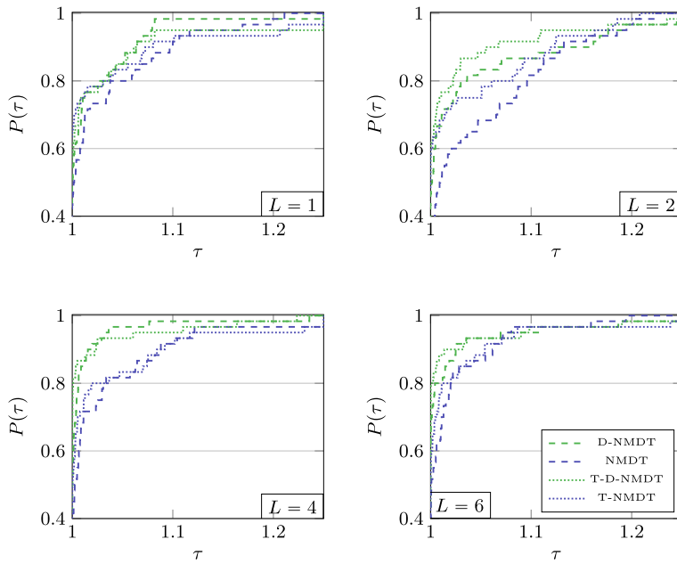
Fig. 5 Performance profiles to dual bounds of NMDT-based methods on sparse instances
