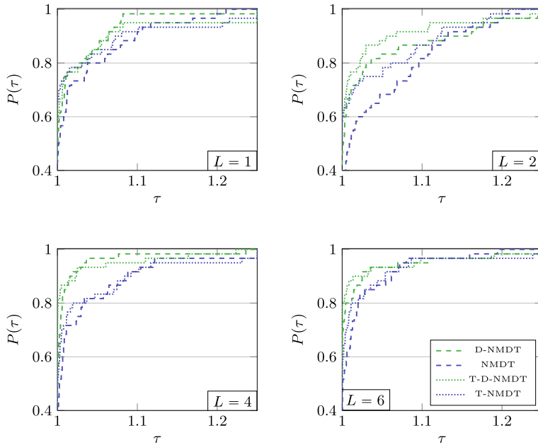
Fig. 6 Performance profiles to dual bounds of NMDT-based methods on dense instances
