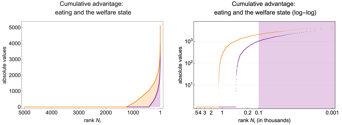
Figure 6: Left: Basic welfare state institutions (orange) in the simple 'people have to eat' model (purple) by changing k = 1.01 to k = 1.005 . Right: Same as left in log-log scale. Both outcomes follow a power law distribution (top 2% for both scenarios; see shading in the right panel).
