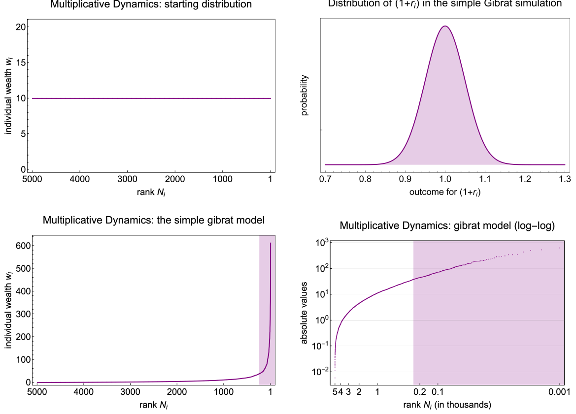
Figure 7: The lower panels will show the typical outcome of a Gibrat model after 1000 turns if random growth rates follow \mathcal{N}(0, 0.05) (as illustrated in the upper right panel) and if all agents start with the same amount of wealth (here w_{i,0} = 10 \forall i as shown in the upper left panel).
