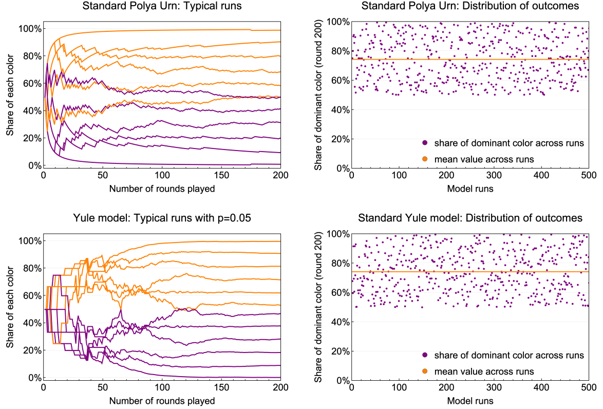
Figure 11: The upper panels show typical outcomes (left) as well as the distribution of outcomes across different runs (right) of the simplest Polya model (with two different colors), while the lower panels illustrate the same for the simplest Yule model (again with n = 2 and reproduction probability of p = 0.05 for each entity in each period). Typical values on left panels are chosen to represent the full spectrum of long-run outcomes for orange as a dominating color.
