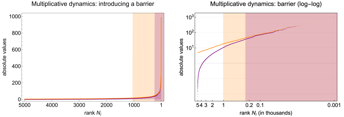
Figure 10: Comparison of the standard Gibrat model with (orange) and without (purple) a barrier at w_{i,t} = 5 (where all agents start with w_{i,0} = 10 ).
