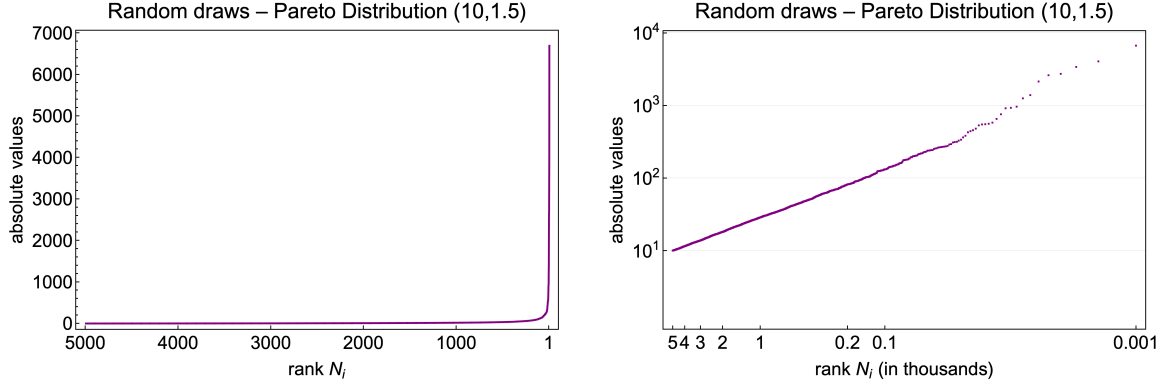
Figure 2: Left: Random draws from a Pareto distribution. Right: The same data in a log-log plot. The largest number is some orders of magnitude larger than the mean, median or any quantile.
