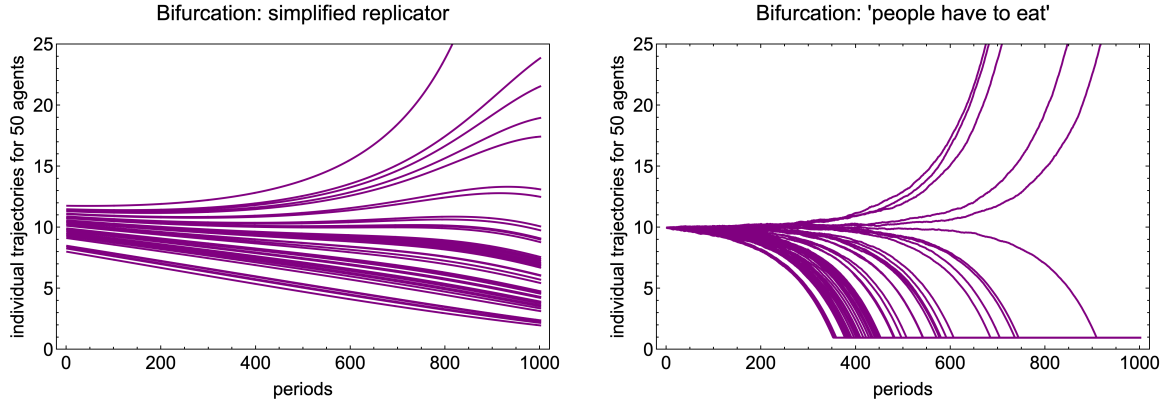
Figure 5: Left: Bifurcation process in the simple replicator model. Right: Bifurcation process in the 'people have to eat' model.
