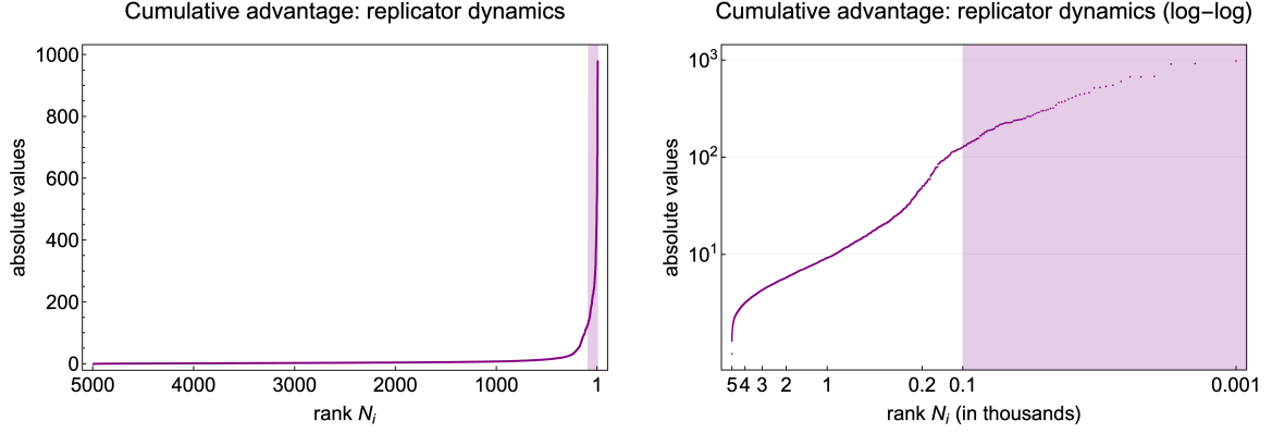
Figure 3: Left: Simulation outcome of a quasi-deterministic cumulative advantage model with k = 1.2 and m = 400 . Right: The same outcome in a log-log plot. Shaded areas follow a power law distribution (top 2%).
