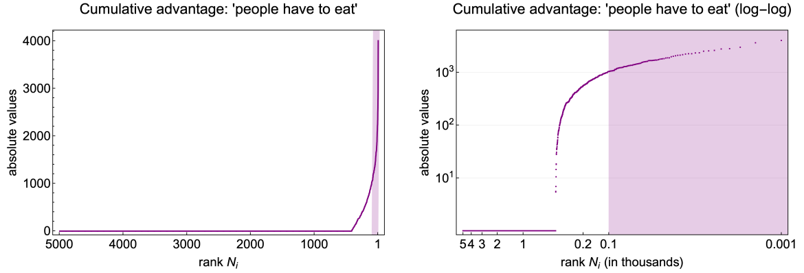
Figure 4: Left: Simulation outcome of a 'people have to eat' model. Right: The same outcome in a log-log plot. Shaded areas follow a power law distribution (top 2%).
