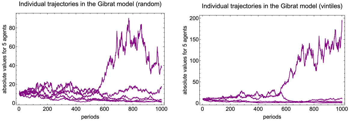
Figure 9: Left: The evolution of wealth for five random agents as sampled from the Gibrat model shown in Figure 7 Right: The evolution of wealth for those five agents that characterize the vintiles of the final distribution of the Gibrat model shown in Figure 7
