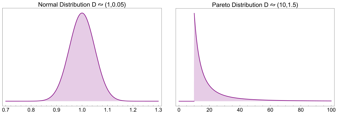
Figure 1: Left: A normal distribution. Right: A power law distribution.
