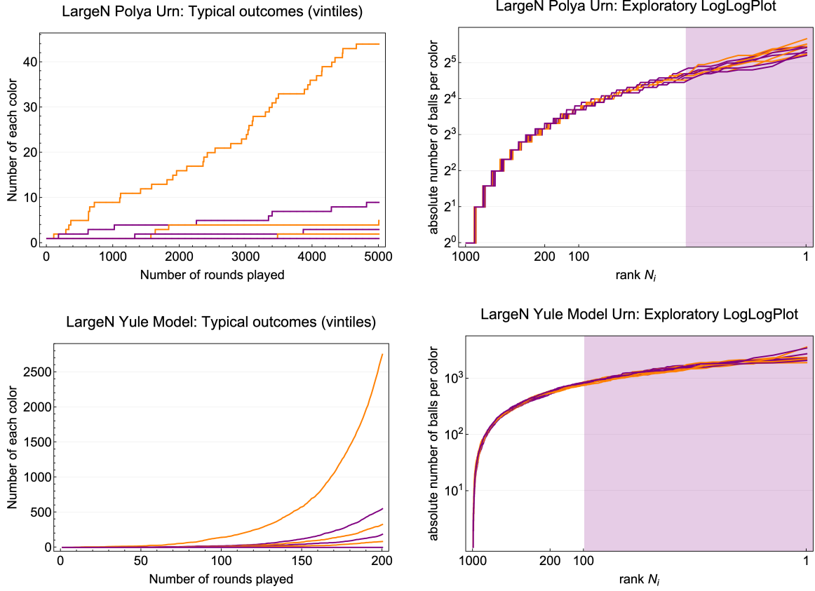
Figure 12: The upper panels show exemplary model runs (left) for a largeN Polya model (with number of colors n = 1000 ) and the final distribution after 5000 rounds for ten different runs (right) in a log-log plot. The lower panels show the same for a largeN Yule model with n = 1000 and reproduction probability of p = 0.03 for each entity in each period. The left panel provides exemplary model runs, the right panel showing the final distribution after 200 rounds again).
