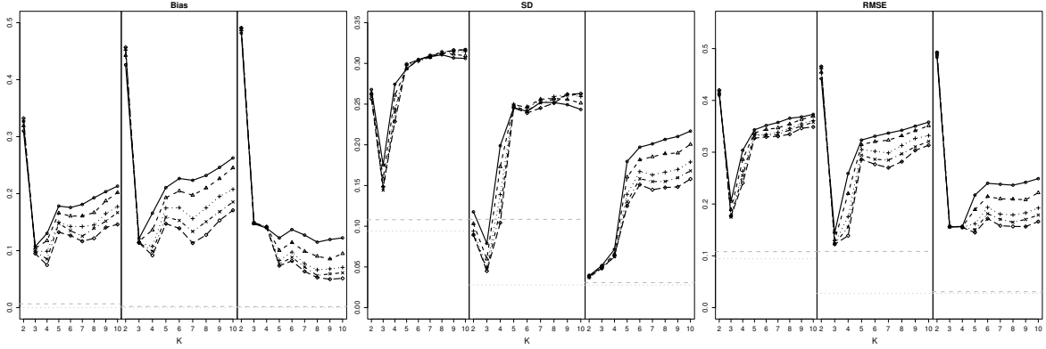
Figure 5.1: Behavior of the Bias, SD and RMSE of the SNPMD estimator for different combinations of K , P , N and M , with respect to II and KF-MLE.
