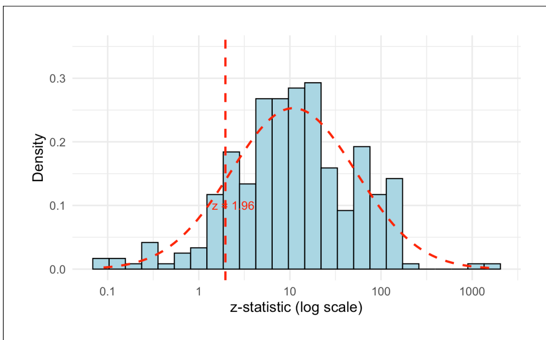
(c) \ln(abs(y_i/se_i))
