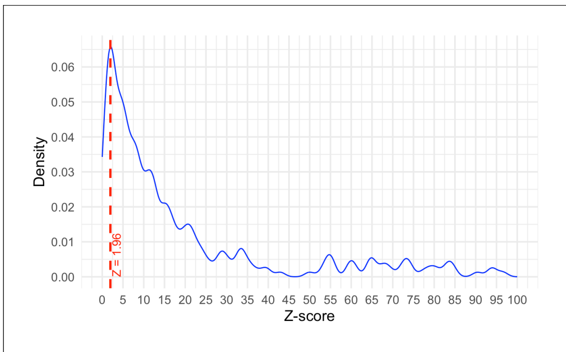
(a) abs(y_i/se_i)
