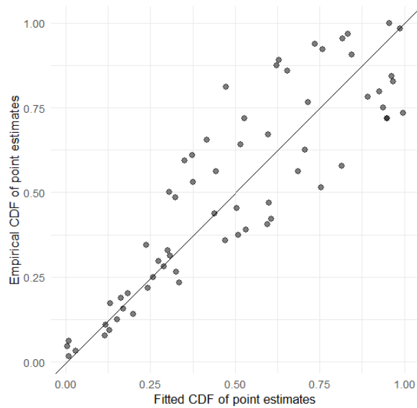
Figure 6: Diagnostic q - q plot: fitted CDF vs. empirical CDF of point estimates
