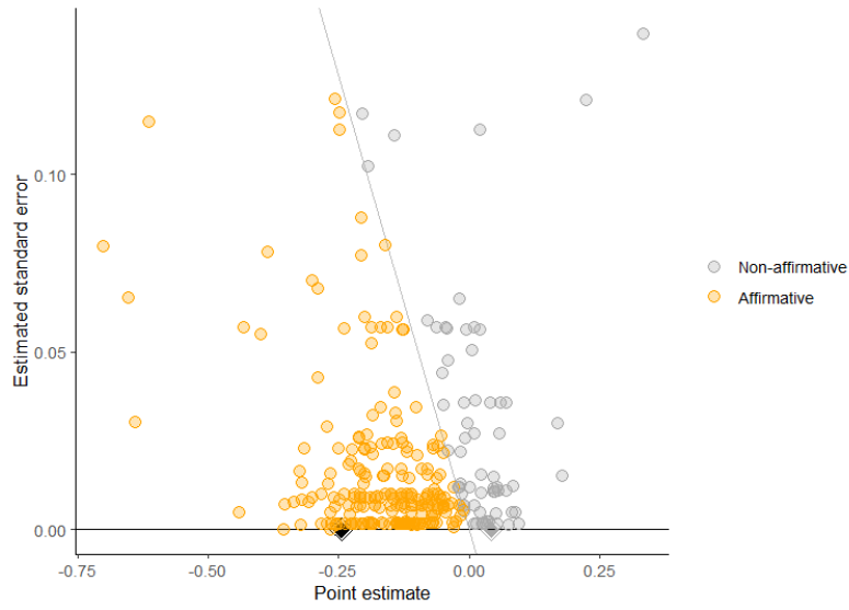
Figure 5: Significance funnel plot
