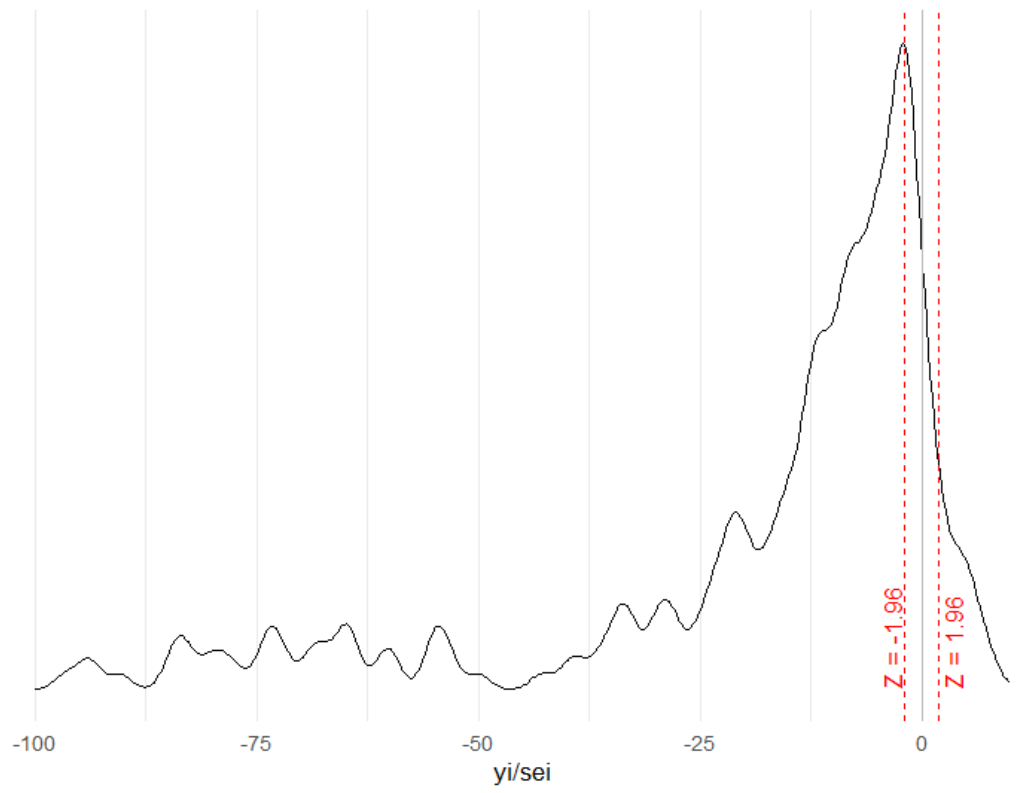
Figure 7: Diagnostic plots: distribution of z -scores
