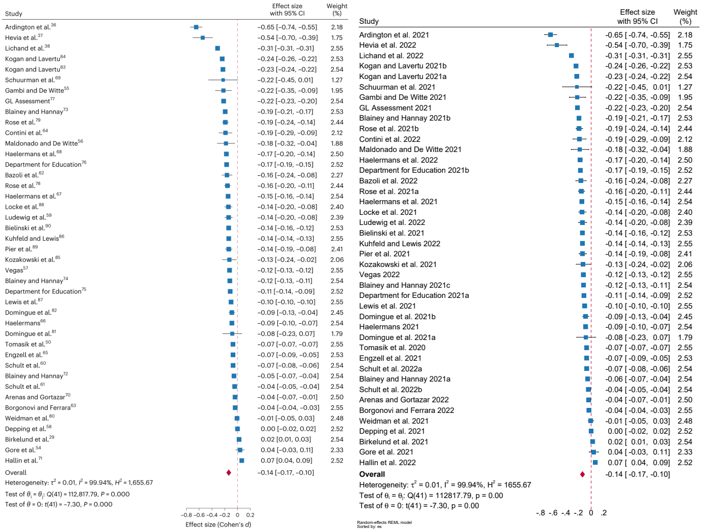
Figure 2: Forest plot
