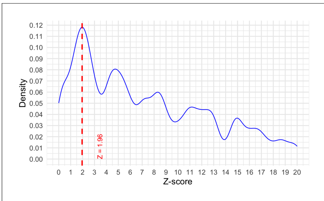
(b) abs(y_i/se_i) zoomed to the (0, 20) neighborhood
