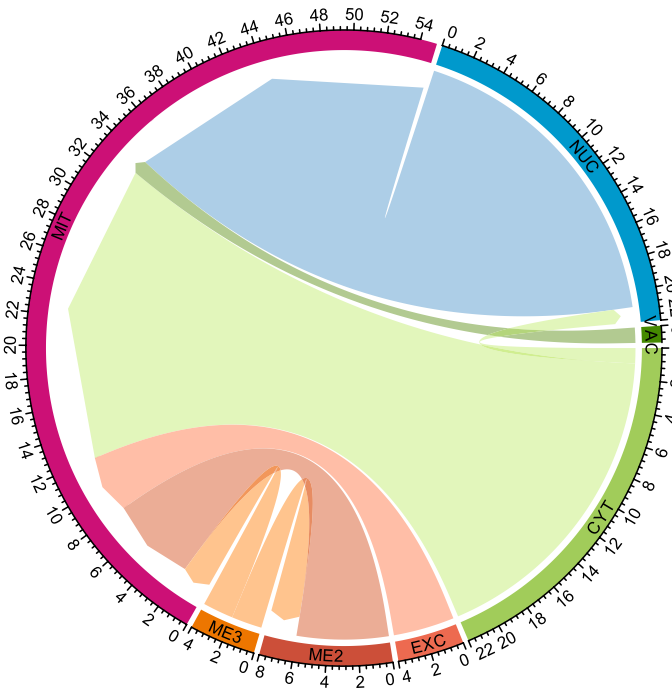
Fig. 13 Changes in prediction when increasing x_{mit} with q_{mit} = \frac{75}{1485} : only observations that switch their prediction portrayed
