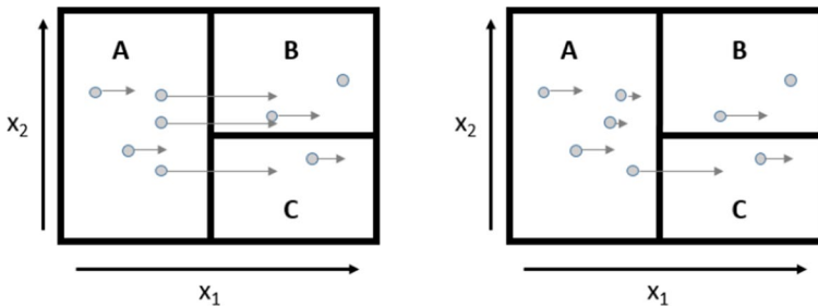
Fig. 10 QSM with q_{x_1} = \frac{1}{n+1} with some equal (left) and slightly jittered (right) data points
