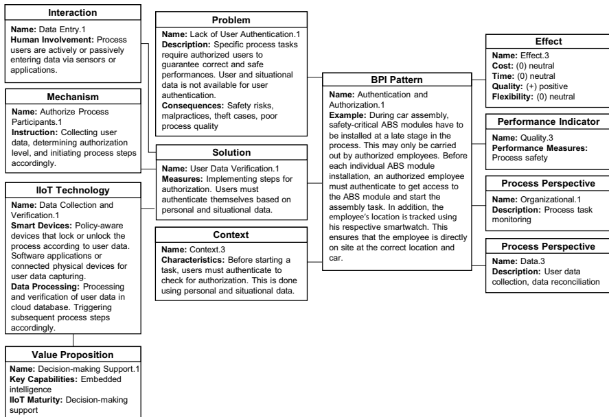
Fig. 9 Authentication and authorization pattern
