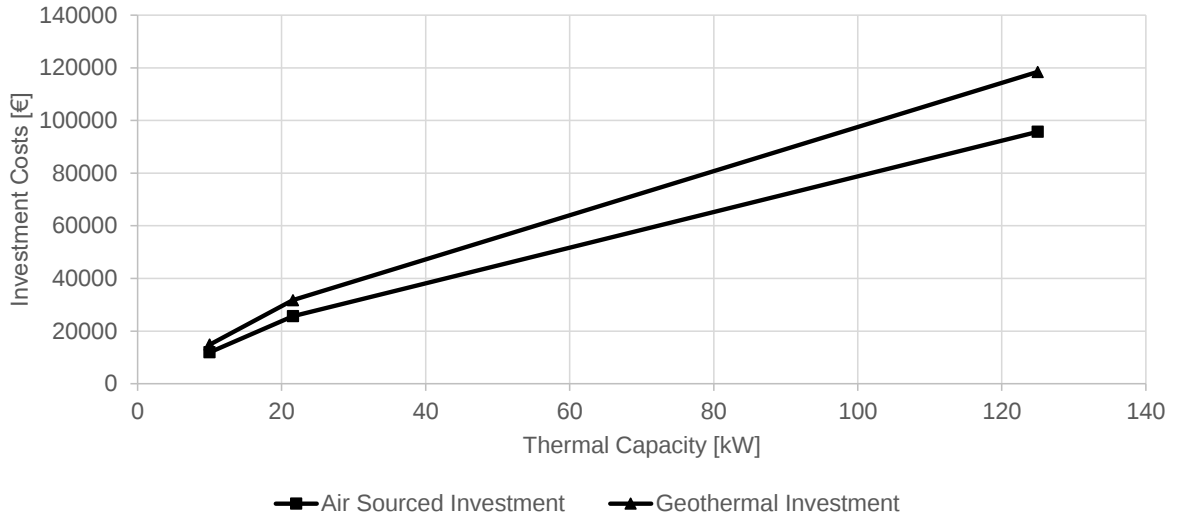
Figure C.4: Investment costs of gas heat pumps in 2020
