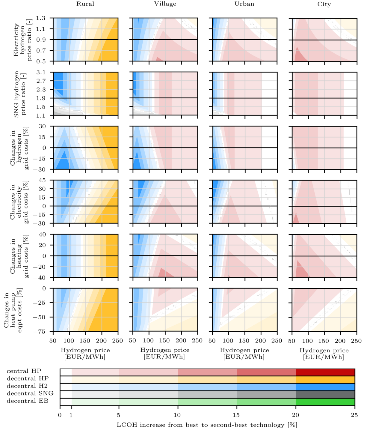
Figure 7: The impact of uncertain and heterogeneous parameters on the cost-efficient heating technology in different settlement types for buildings with a supply temperature of 30°C. Colors indicate the cost-efficient technology. Color shades indicate the LCOH increase from the cost-efficient to the second-best technology. Black lines show the baseline assumption of each varied parameter.
