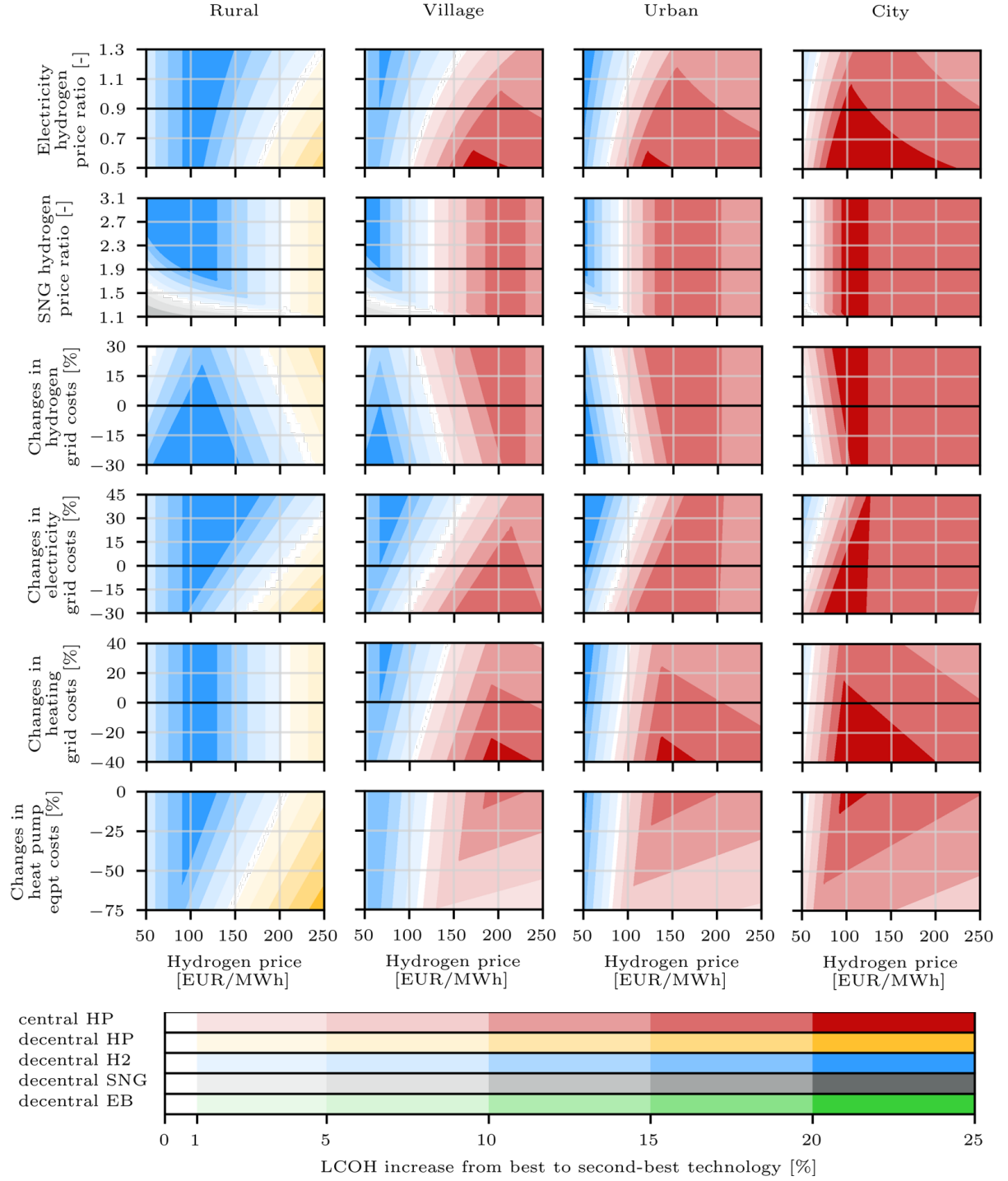
Figure 6: The impact of uncertain and heterogeneous parameters on the cost-efficient heating technology in different settlement types for buildings with a supply temperature of 70°C. Colors indicate the cost-efficient technology. Color shades indicate the LCOH increase from the cost-efficient to the second-best technology. Black lines show the baseline assumption of each varied parameter.
