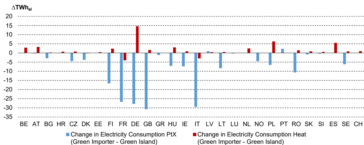
Figure E.10: Change in the resulting electricity consumption from ptx technologies and heaters between the Green Importer Europe scenario and Green Island Europe scenario in 2050
