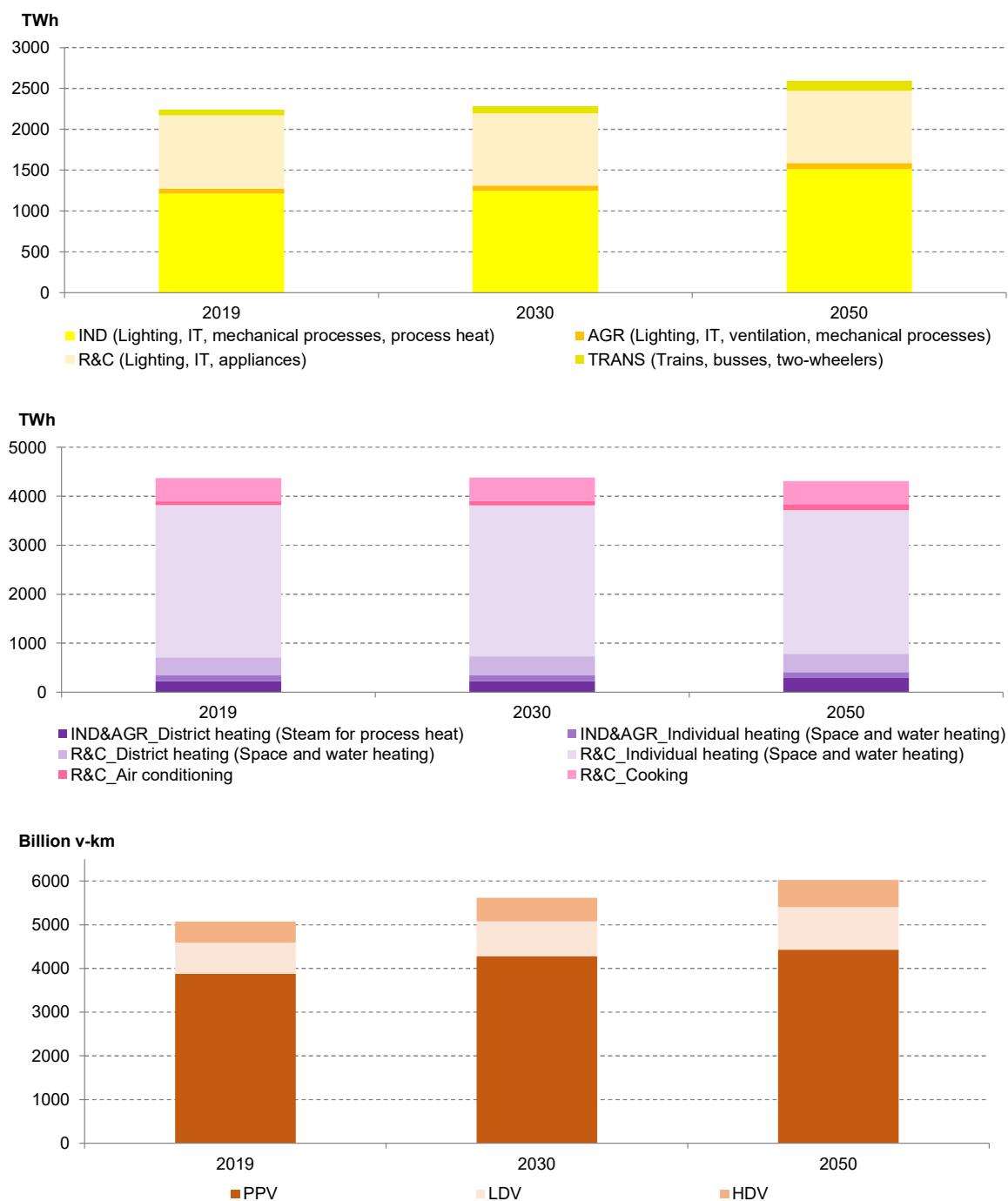
Figure C.3: Assumptions on the development of useful and secondary electricity demand (top), useful heat demand (middle) and useful demand for vehicle kilometers (bottom) in the end-use sectors in Europe up to 2050 (own assumptions based on Mantzos et al. (2019), dena et al. (2021) and Helgeson and Peter (2020))
