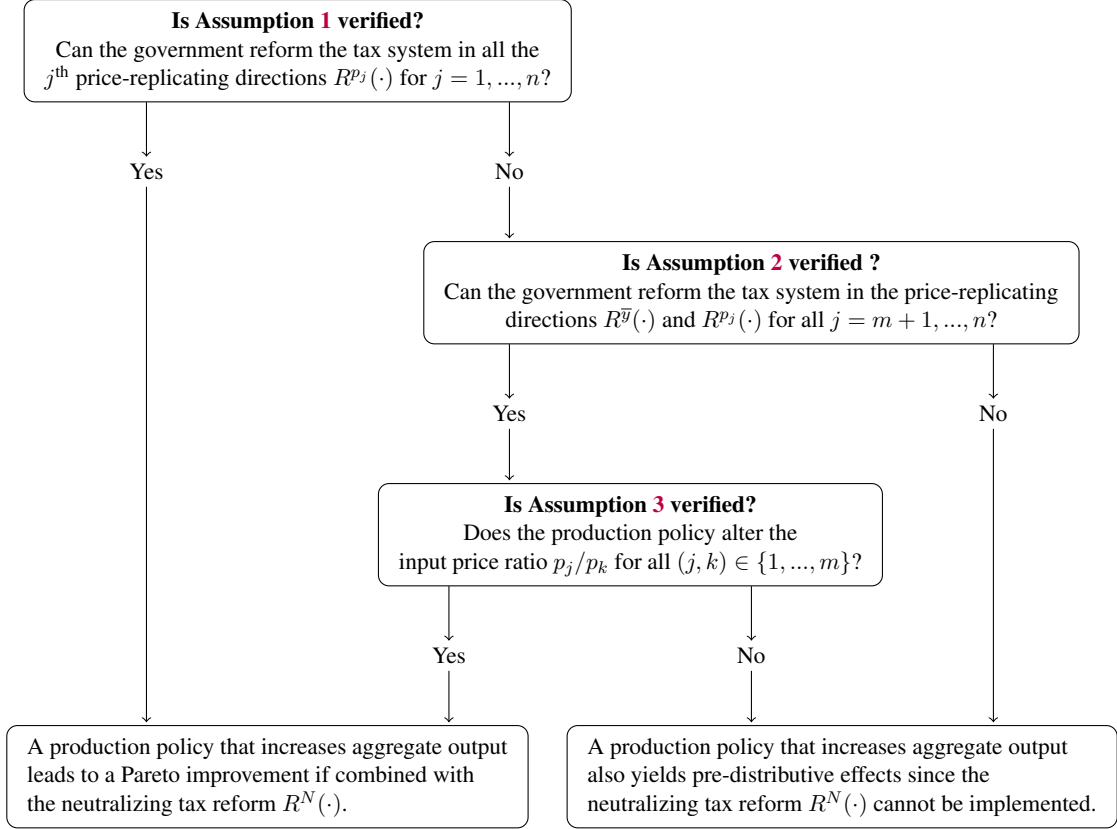
Figure 2: Decision Tree
