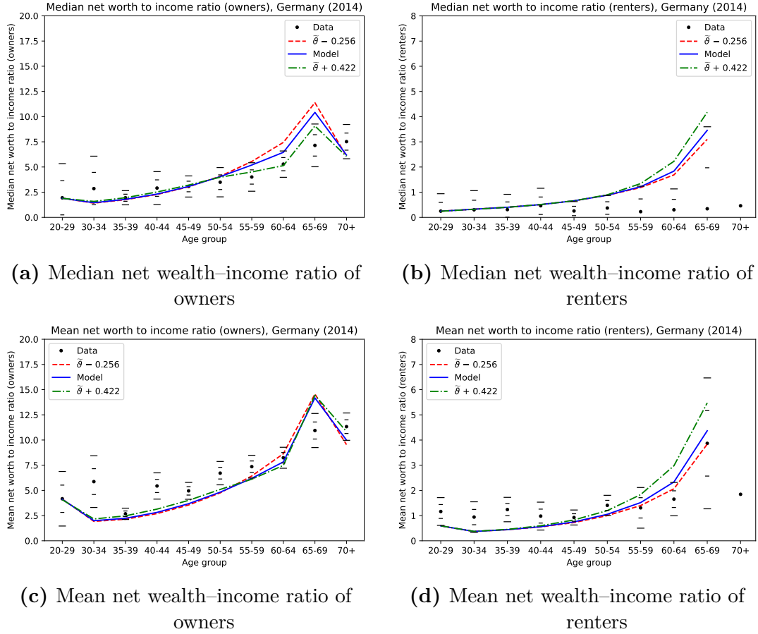
Figure 13 Identification of the Spread of the Discount Rate \tilde{\vartheta}
