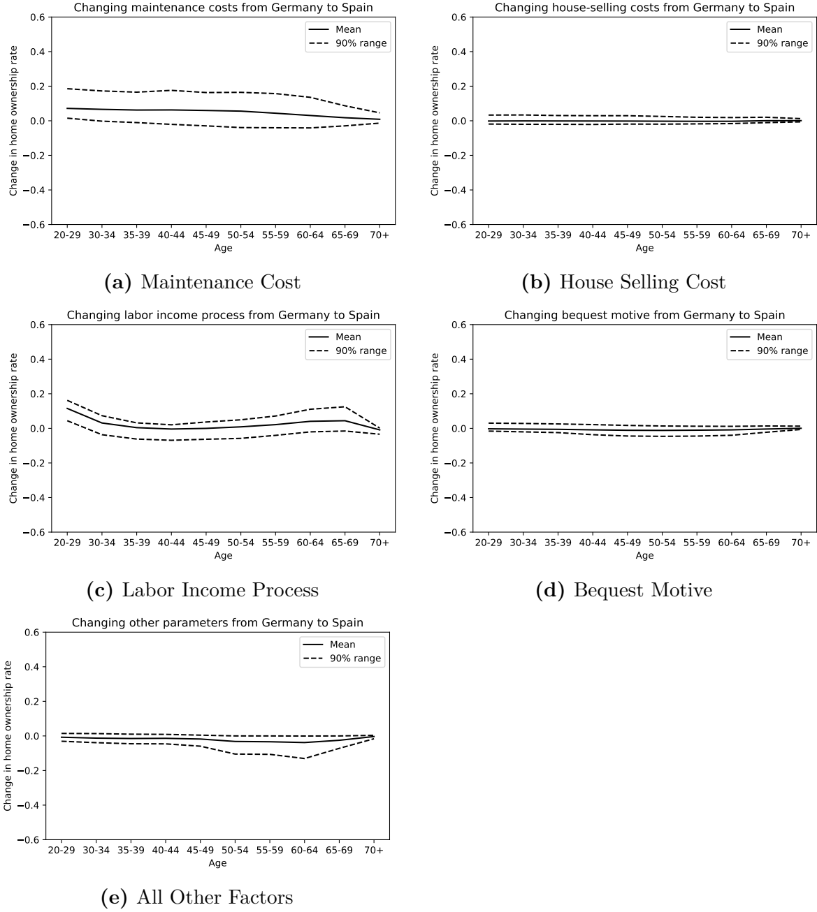
Figure 20 Decomposition of Homeownership Rates: Germany \rightarrow Spain II.
