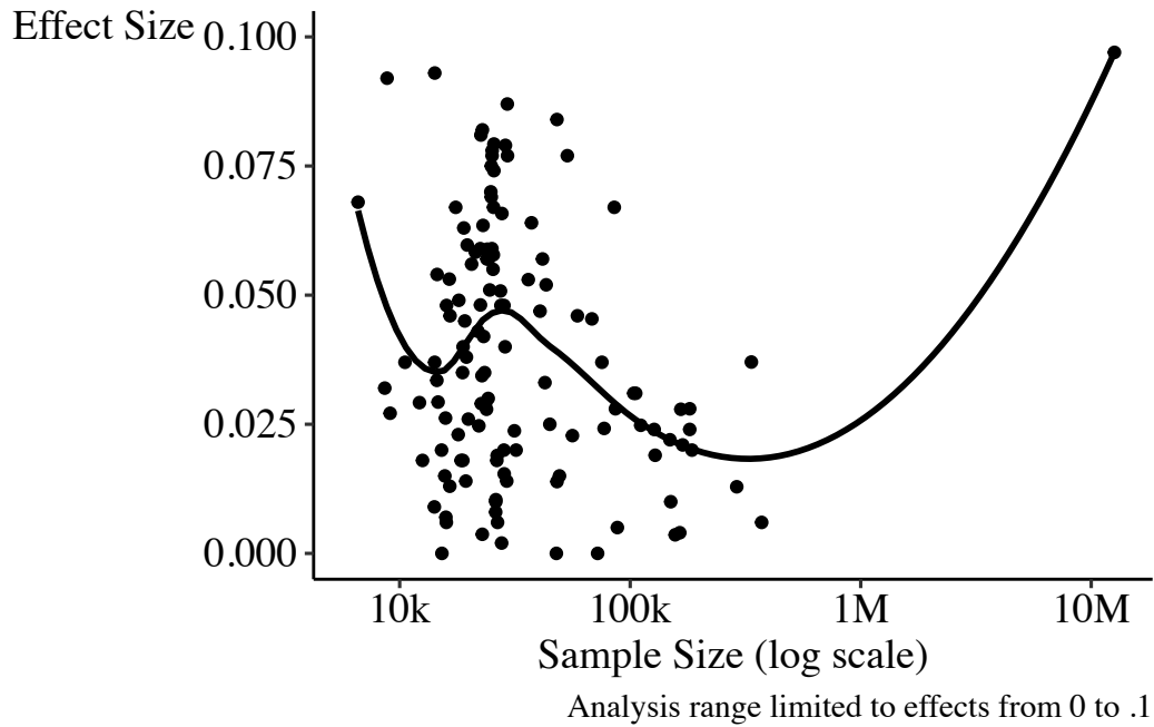
Figure C.2: Task 2 Effect Size and Sample Size
