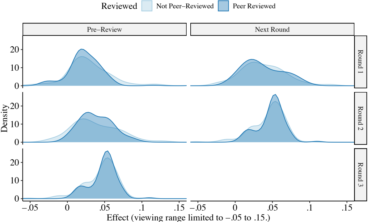
Figure D.1: Distributions of Reported Effect Sizes
