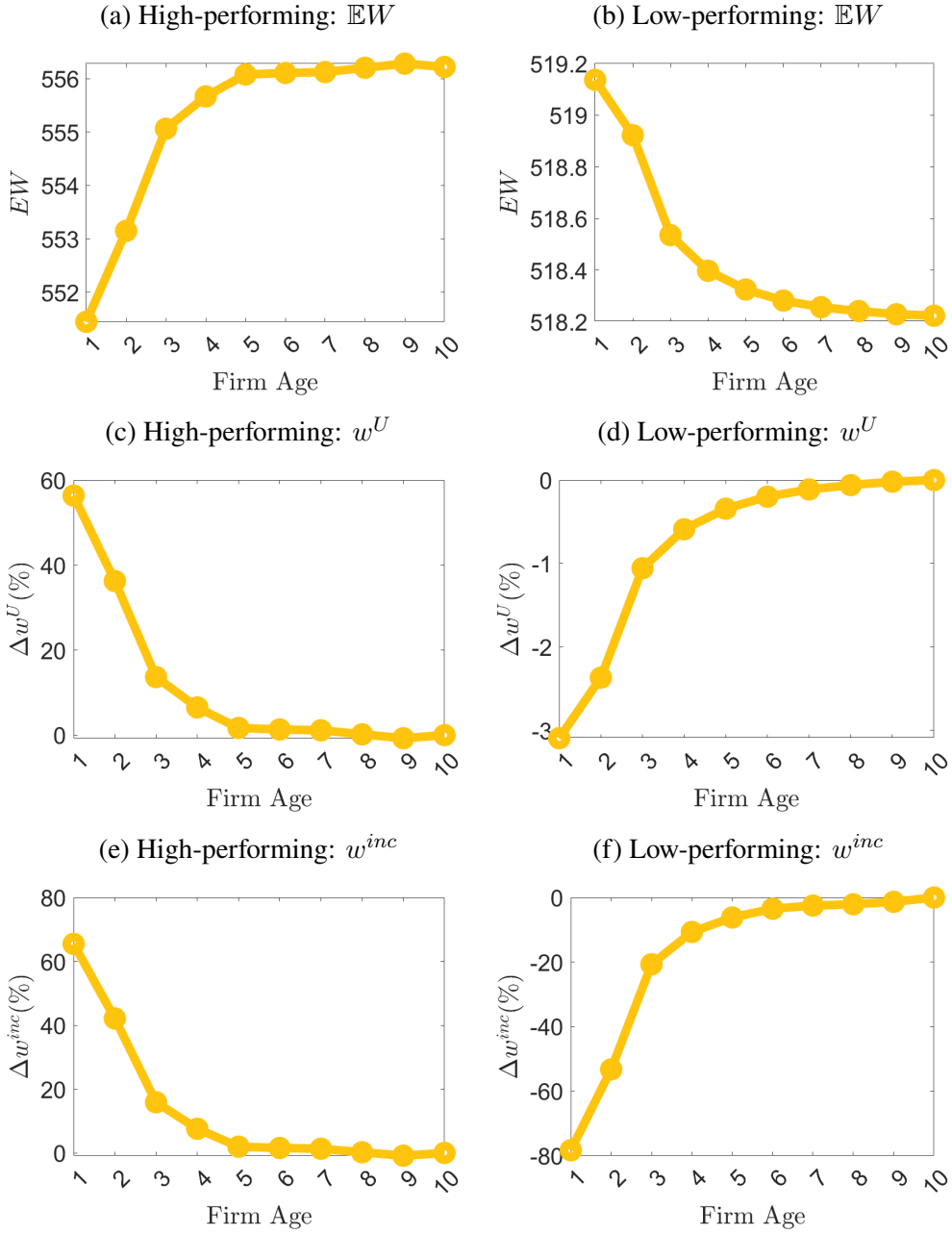
Figure 3: High vs. Low-performing Firms
