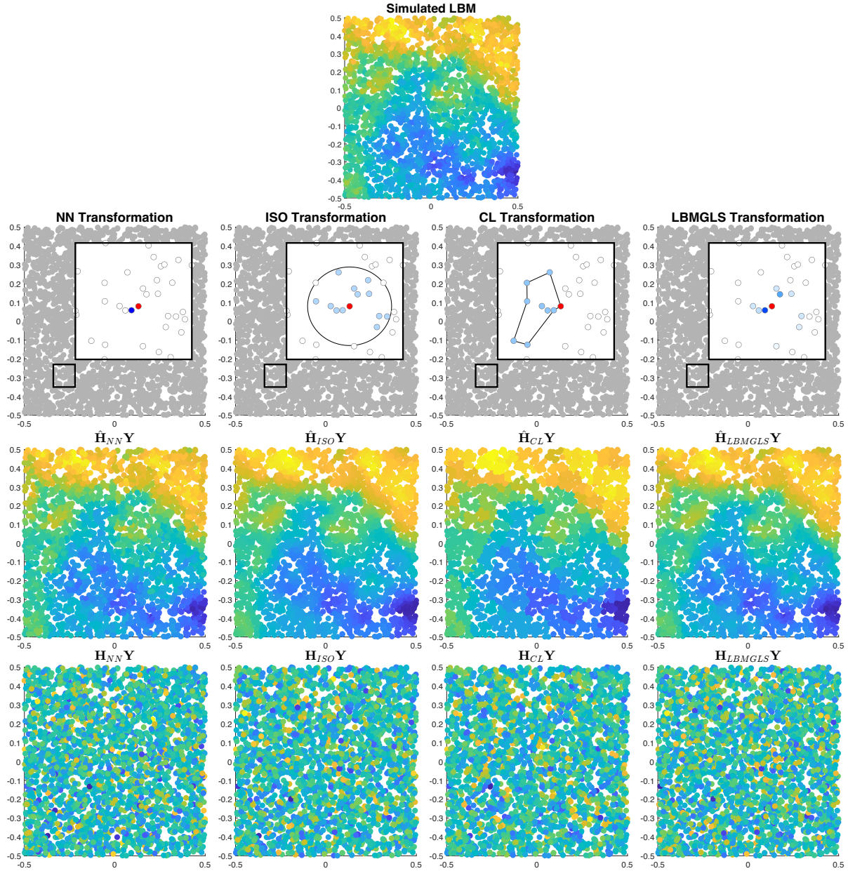
Figure 4: Differencing transformations
