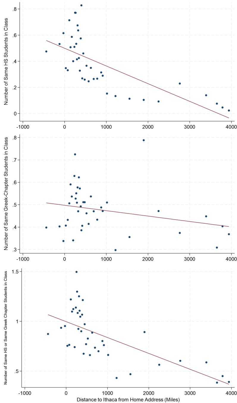
Figure 5: Binscatter Plot Friendship in Class and Distance from Home Address Among Freshman Students
