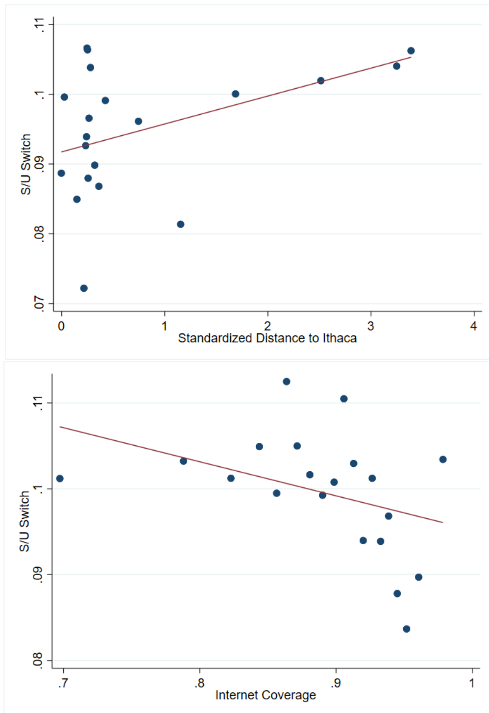
Figure 3: S/U Switch by Standardized Distance to Ithaca and by Internet Coverage
