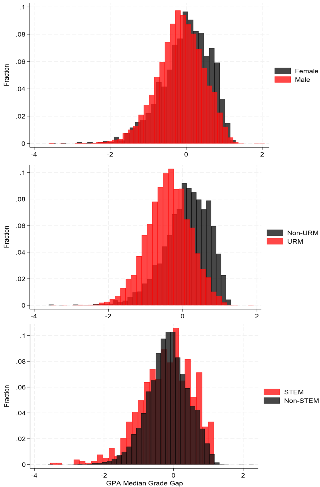
Figure 4: GDP Median Grade Gap Distribution by Gender, URM and STEM Major
