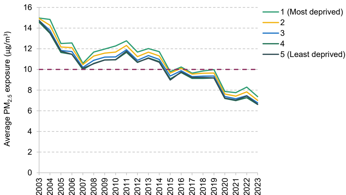
Figure A1. Average PM 2.5 exposure over time by income deprivation quintile in 2004
