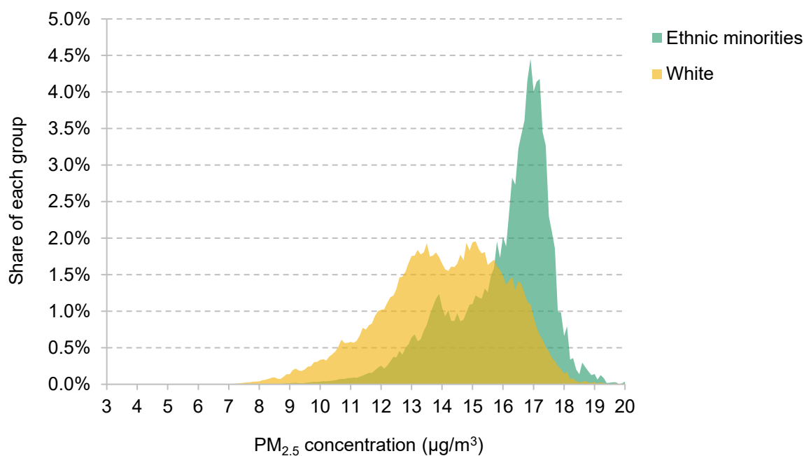
Figure A3. Distribution of PM 2.5 exposure in 2003–04, by ethnicity
