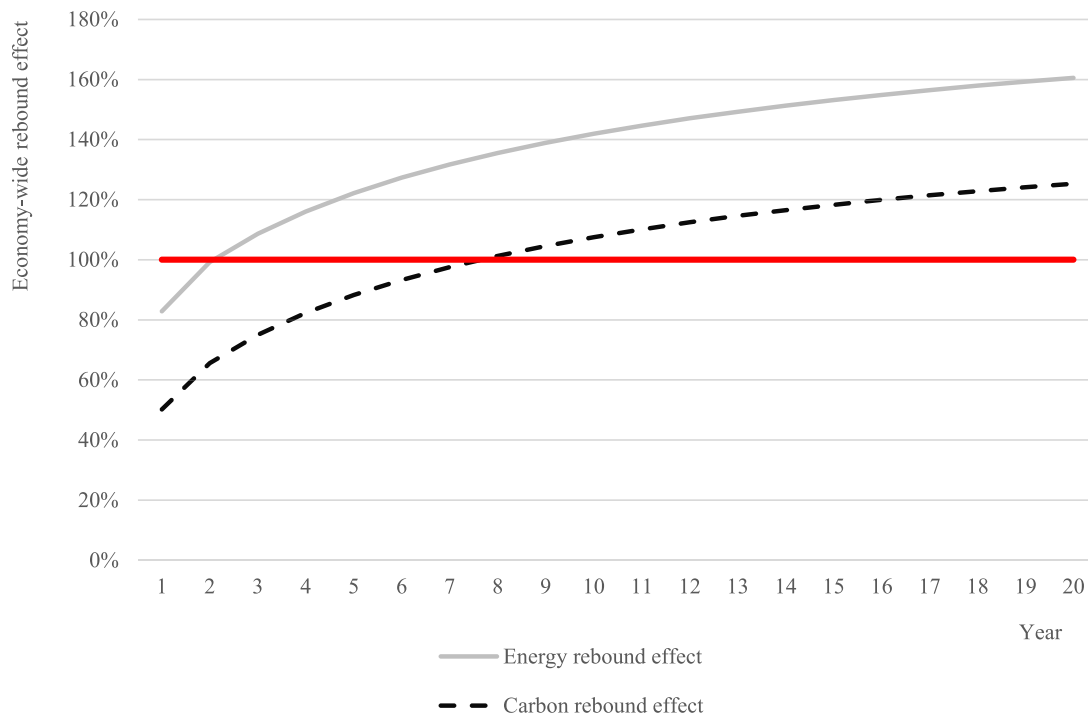
Fig. 2. The economy-wide rebound effect of the Catalan economy each year of the simulation.
