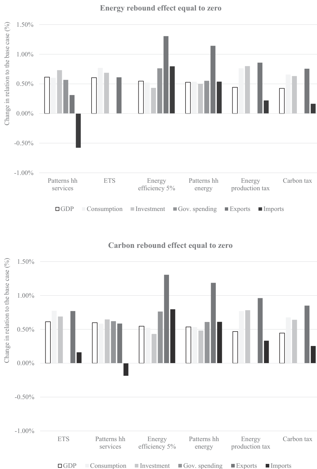
Fig. 7. Average of yearly values for the 20-year period simulation of the GDP variation (in relation to the base case) and its components for the different scenarios.
