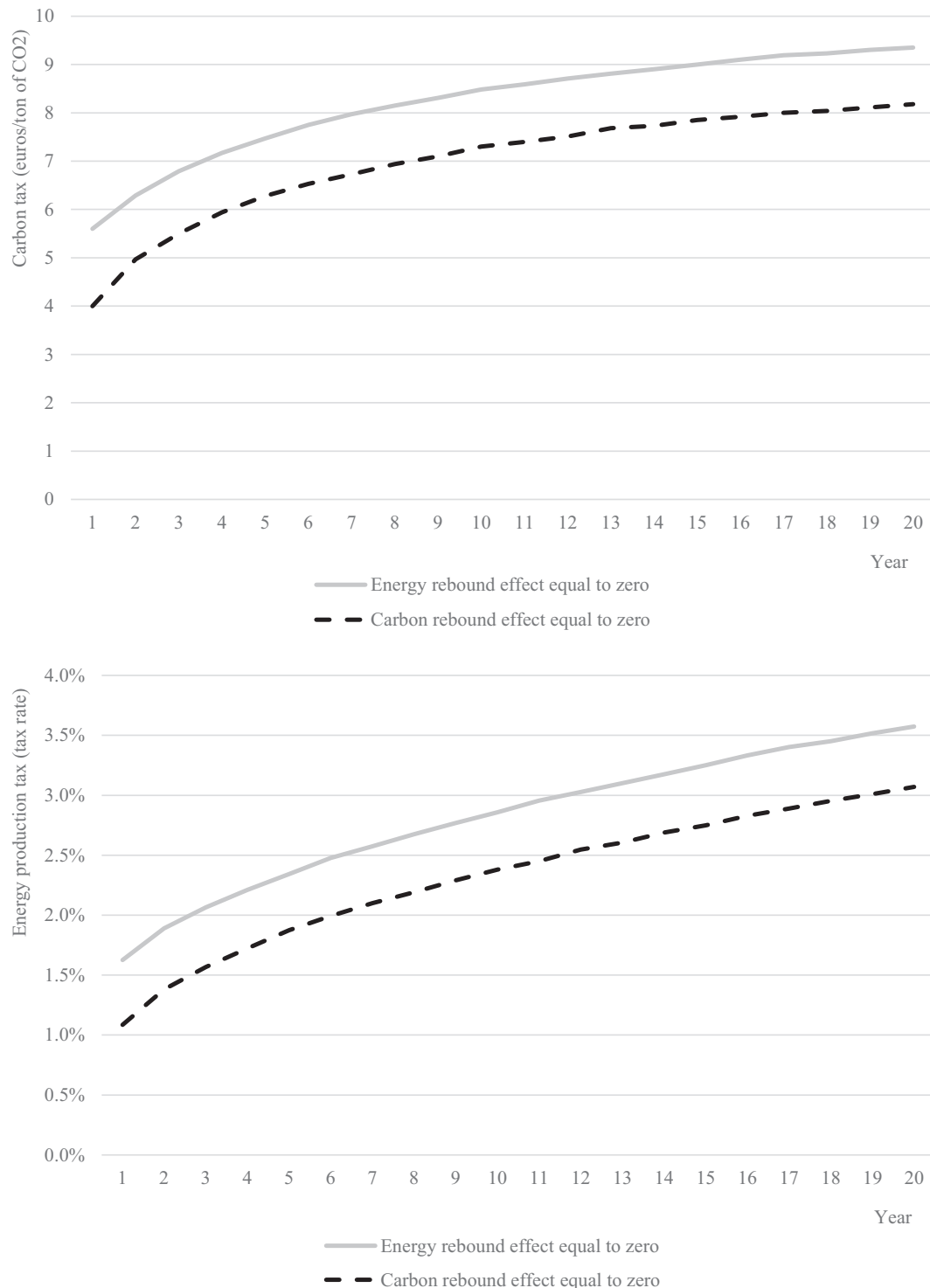
Fig. 3. Carbon and energy production taxes that totally offset energy and carbon rebound effects each year of the simulation.
