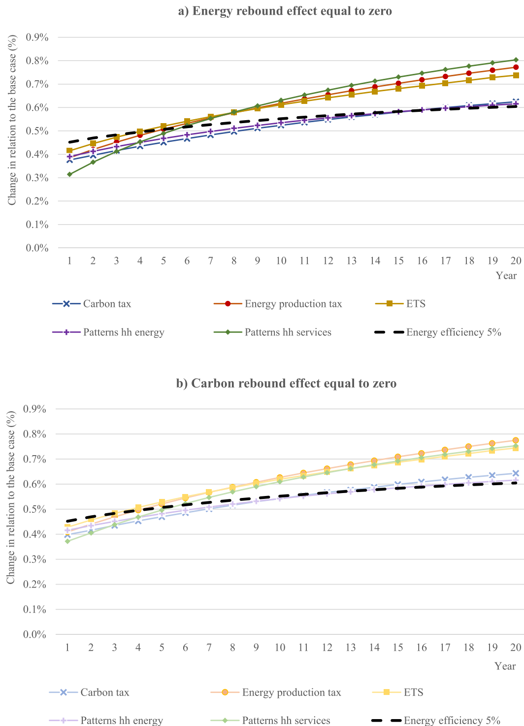
Fig. 6. GDP variation of different scenarios over the 20-year period of the simulation, in relation to the base case. Note: Patterns HH energy: reduction in energy consumption; patterns HH services: increase in services consumption.
