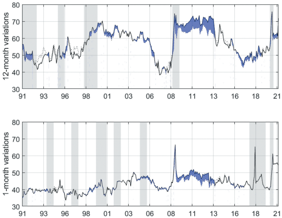
Figure A3. Total connectedness (%), 5 year rolling window, 12- and 1-month IPI variations. Note: the solid line was obtained with the IPI and the dotted line with the idiosyncratic components. The blue area indicates the difference among them, which is interpreted as the common factor. The gray bars correspond to the regional crises estimated with the MS-VAR model.
