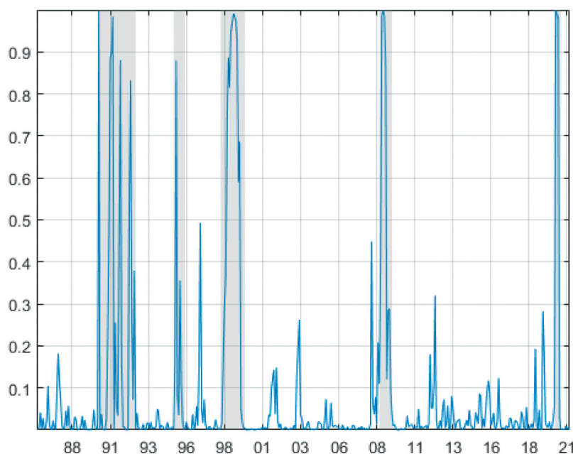
Figure 3. Regional recession probabilities. Note: estimates obtained with the MS-VAR model.
