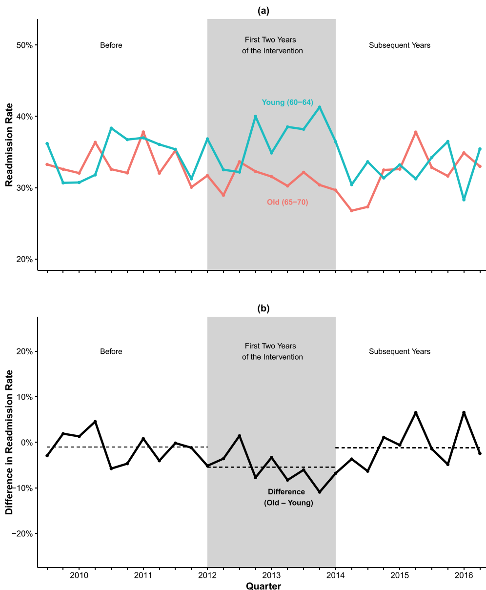
Figure 1. Readmission rates by age group over time, high-risk patients. N = 19,453 admissions from 2010 to 2016 with predicted readmission risk score of 50 or more (top 13% of the risk distribution, mean readmission rate 33%). Panel (a) shows quarterly 30-day readmission rates for patients aged 65–70 (Old) and 60–64 (Young). Panel (b) shows the difference in readmission rates between these age groups. The horizontal-dashed lines in panel (b) mark the average difference for each of the three periods studied. This difference is statistically significant for the first 2 years after the program start (See Table 4). Results for all admissions are shown in Figure A7. Source: authors' calculations using Clalit Health Services data.
