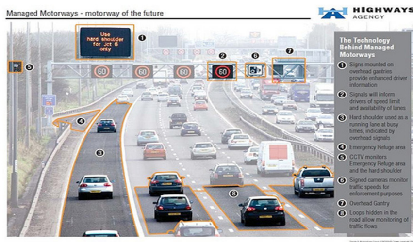
Figure 7: An illustration of active traffic management
