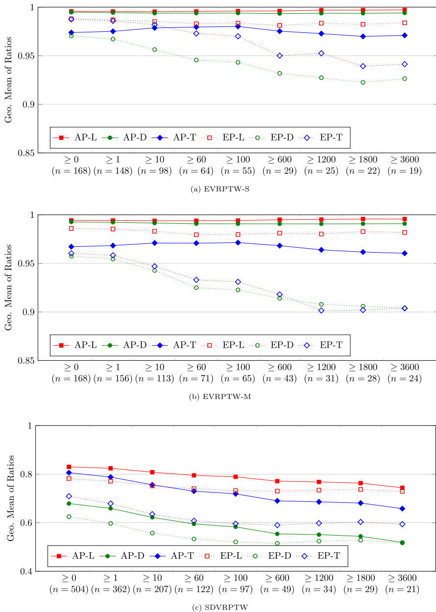
Fig. 5 Geometric mean of ratios of the number of created labels (-L), the number of dominance tests (-D), and the solution time (-T) for either all pricing problems solved (AP) or only exact pricing over the full network (EP). Results are grouped according to total runtimes \geq t
