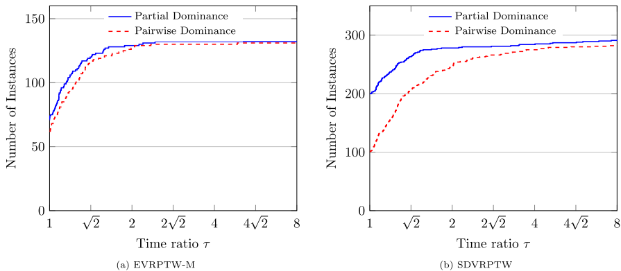
Fig. 6 Performance profiles of individual runs of the BPC algorithms with partial dominance and with only classical pairwise dominance. Note that the abscissa has a logarithmic scale
