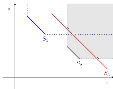
(a) Impact of the order in which S_1 and S_2 are compared with S_3 when partial dominance over a central piece is not performed.
