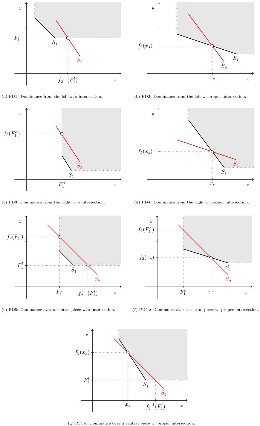
Fig. 3 Different cases of partial dominance
