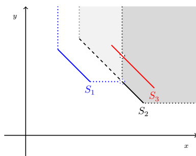
(b) Impact of double bookkeeping when S_1 is first compared with S_2 and afterwards S_2 is compared with S_3 .
