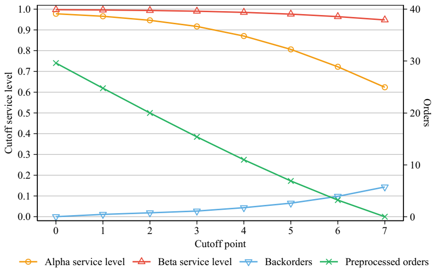
Fig. 7 Performance measures SL_\alpha , SL_\beta , \mathbb{E}[M] , \mathbb{E}[P] depending on cutoff point \tau_C for an exemplary order fulfilment process ( U = 0.8 , scv[D] = 0.5 , scv[B] = 0.5 ); given time-independent customer demand
