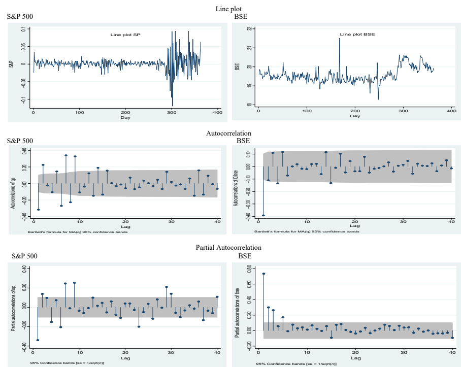
Figure 3. Line plot, ACF, PACF of S&P 500 and BSE time series data
