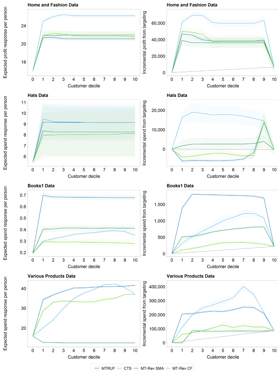
Fig. 3 MT-Rev Analysis for Data Sets 1–4
