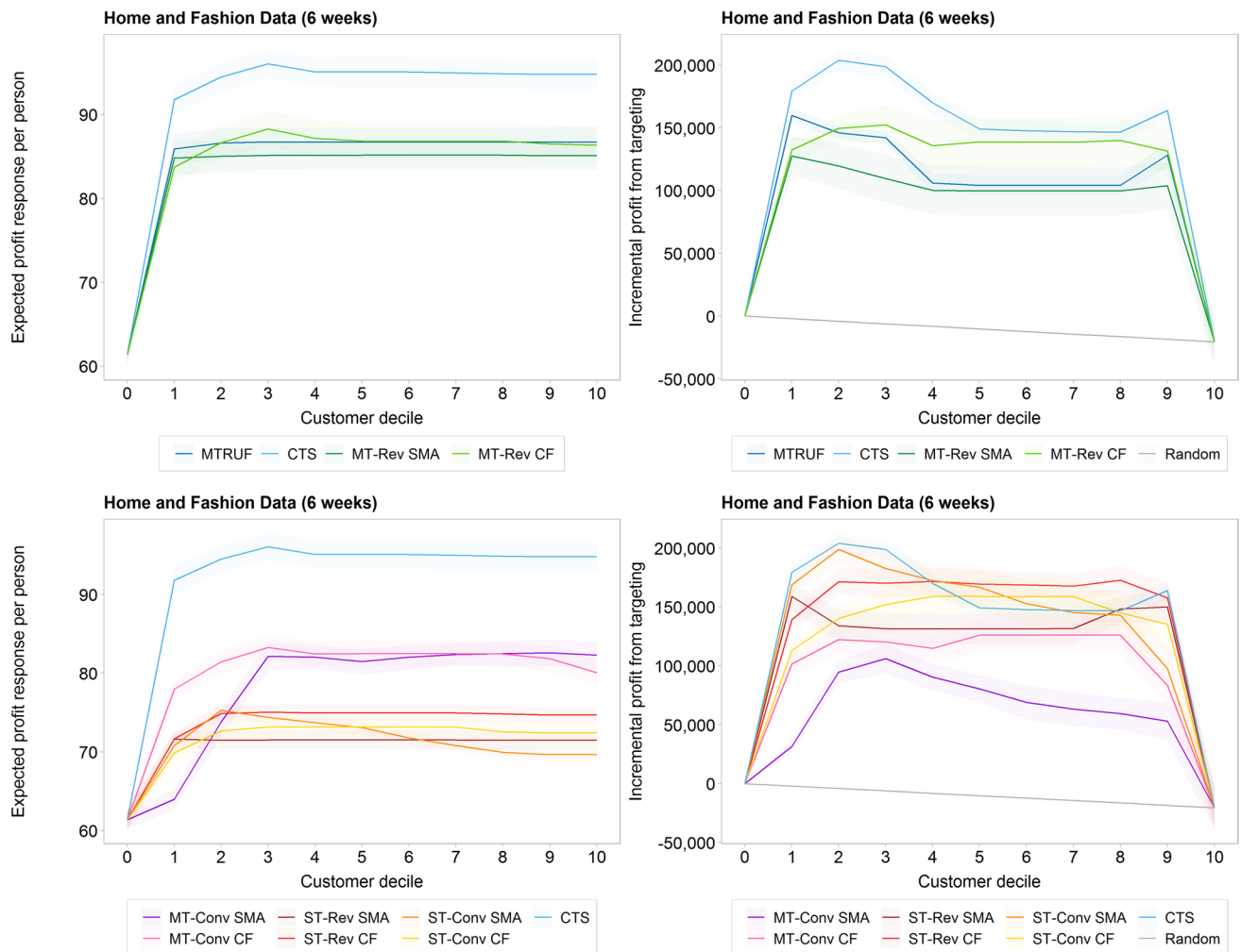
Fig. 7 Model Analysis for a Six-Week Post-Campaign Period
