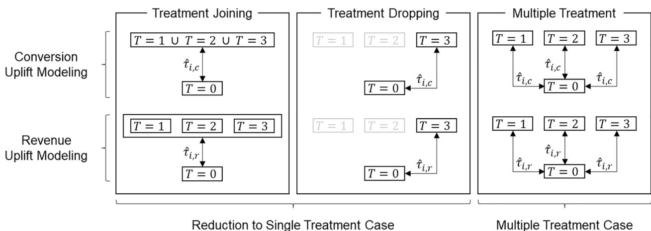
Fig. 2 Approaches to Operationalize the Modeling Settings
