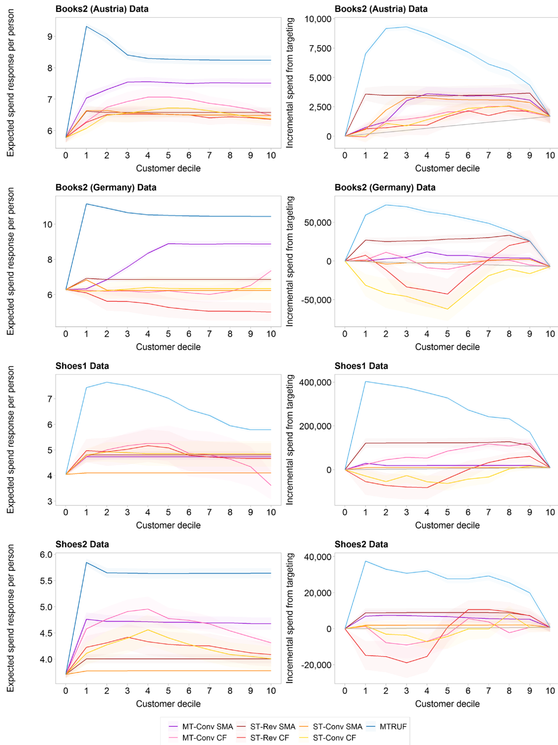
Fig. 6 Analysis of MT-Rev vs. Other Settings for Data Sets 5–8
