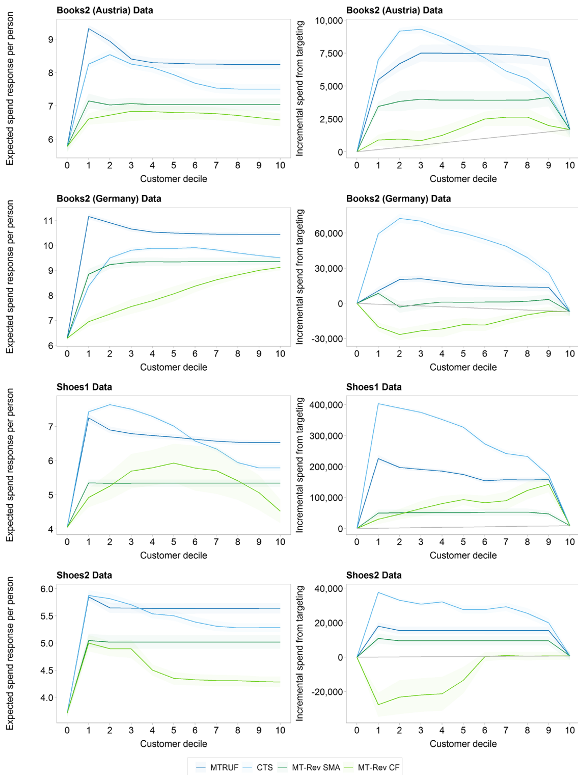
Fig. 4 MT-Rev Analysis for Data Sets 5–8
