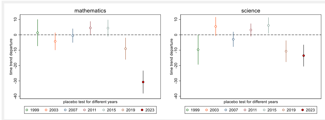
Figure 2: Placebo tests
