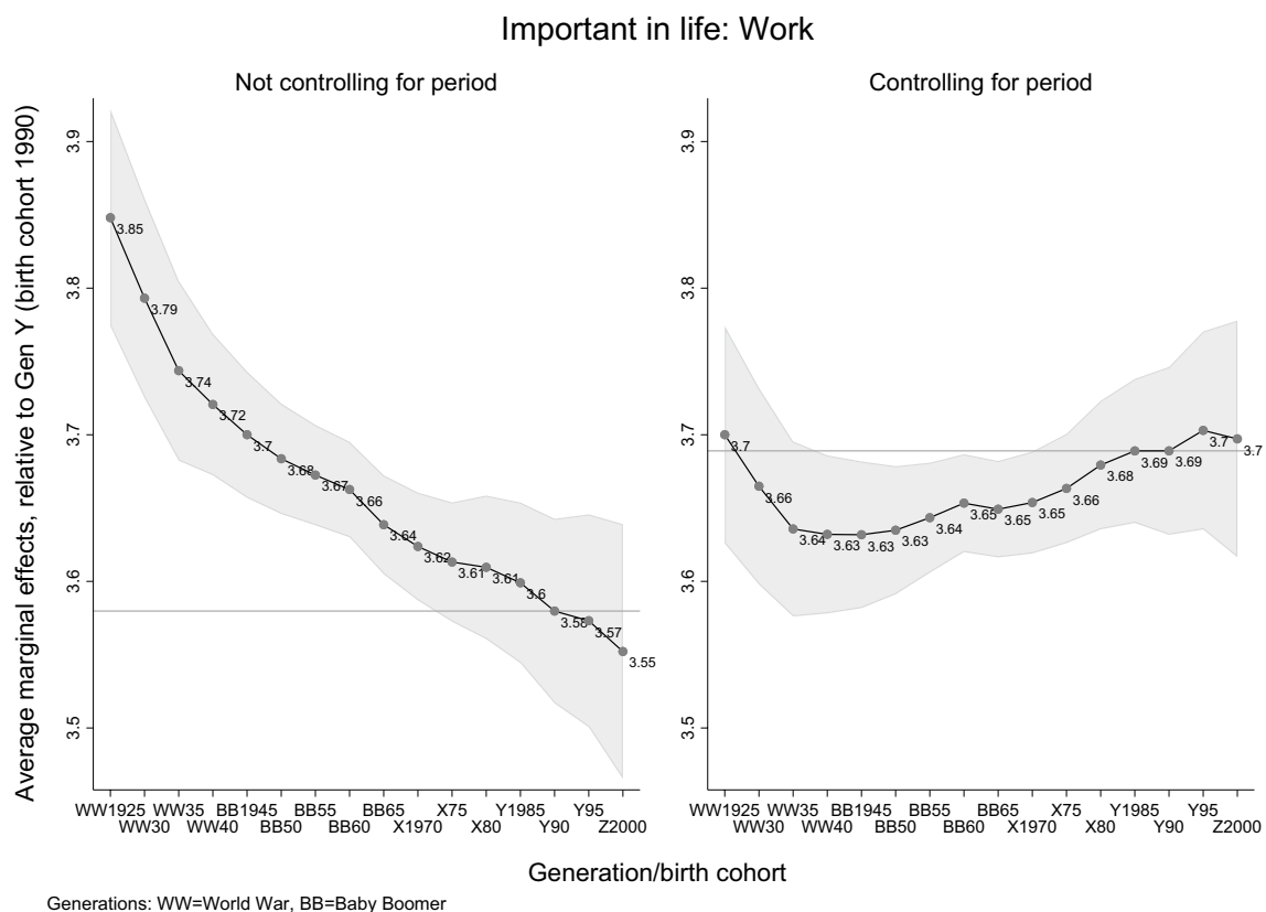
Fig. 1 Importance of work before controlling period effects (left) and after (right)
