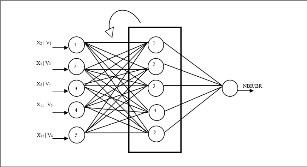
Figure 5 An Architecture of Recurrent Neural Networks in Research Approach R1 and R2
