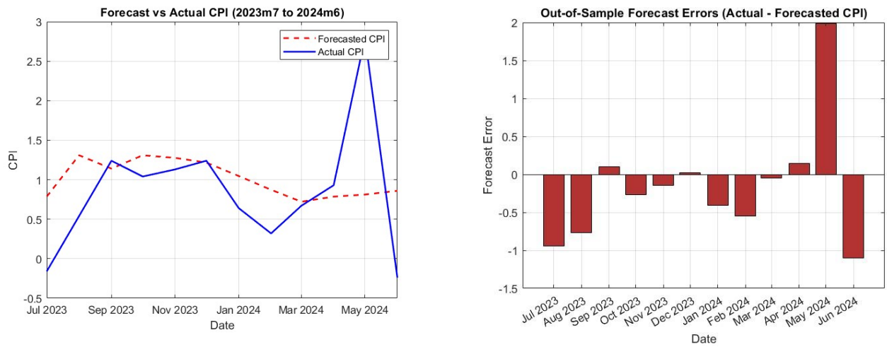
Graph 19. FAVAR with lag 4
