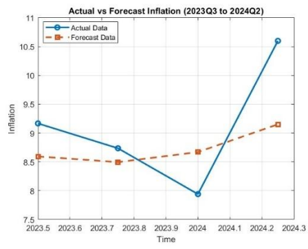
Graph 9. BVAR-7 with lag 1
