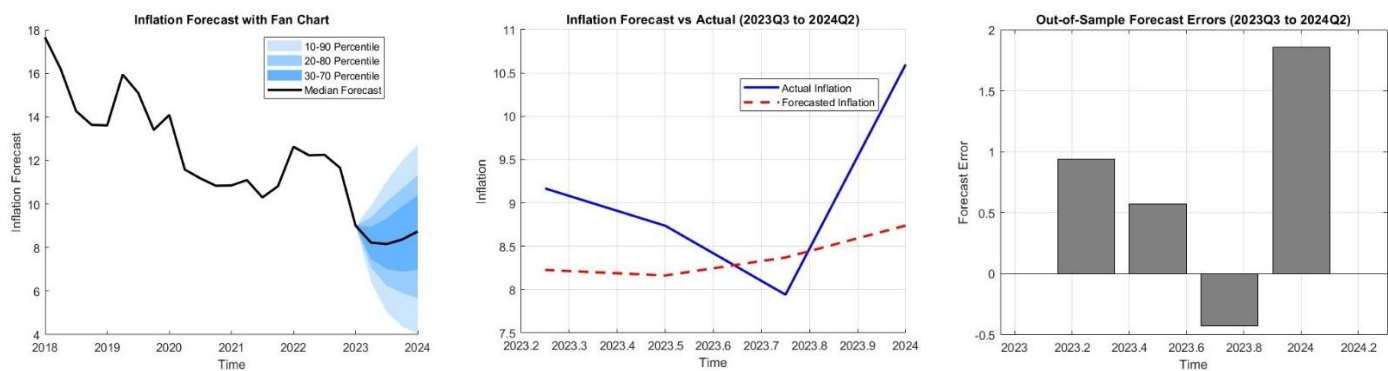
Graph 3. Bayesian AR with lag 3
