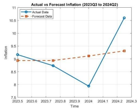
Graph 6. BVAR-5 with lag 2
