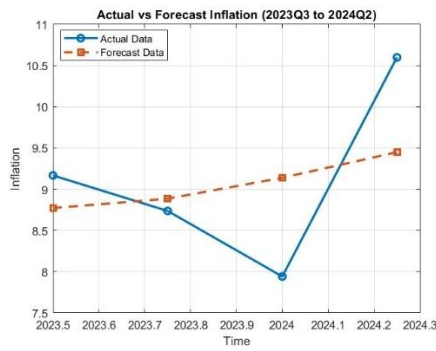
Graph 6. BVAR-5 with lag 2
