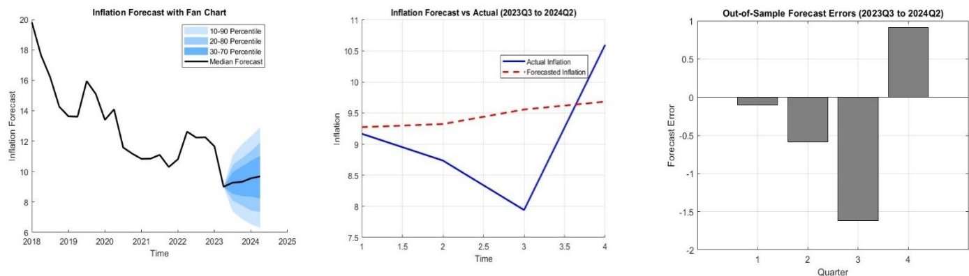
Graph 2. Bayesian AR with lag 2
