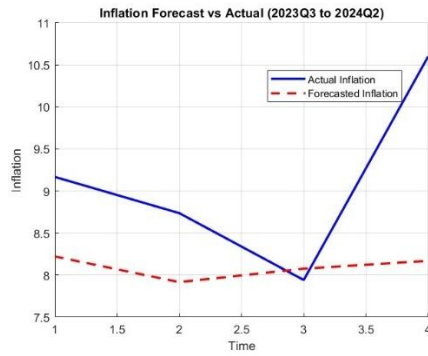
Graph 5. BVAR-5 with lag 1
