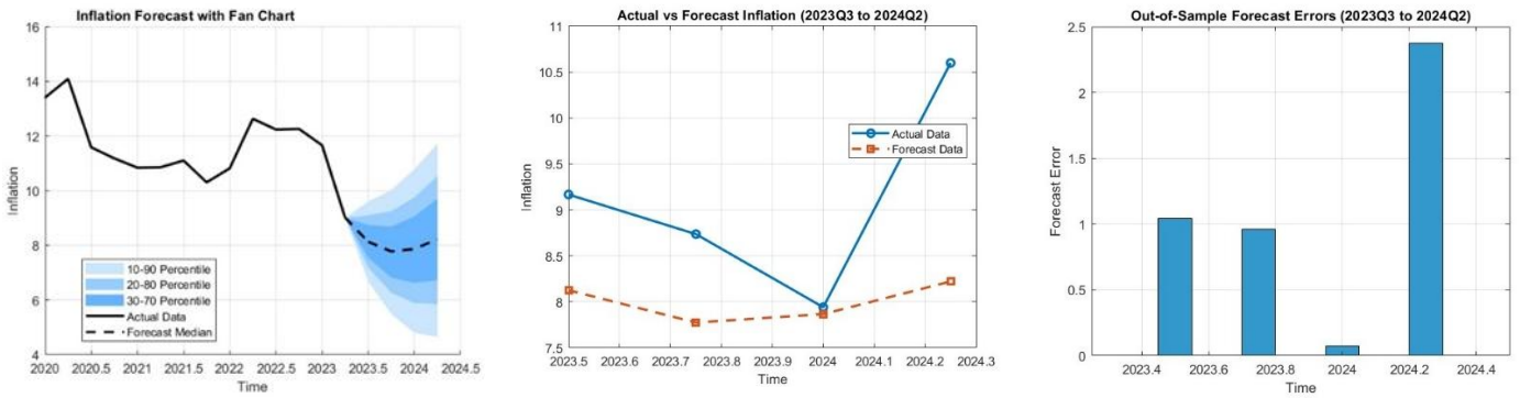
Graph 15. BVAR-10 with lag 3
