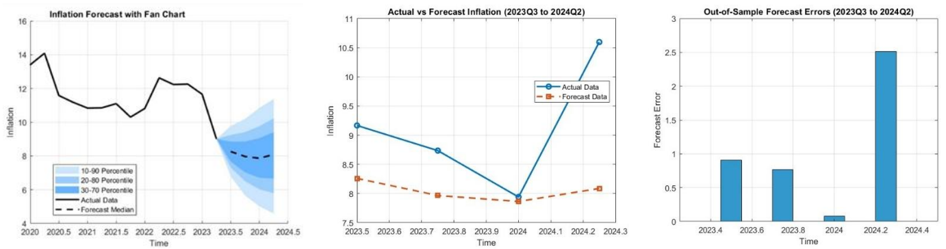
Graph 14. BVAR-10 with lag 2
