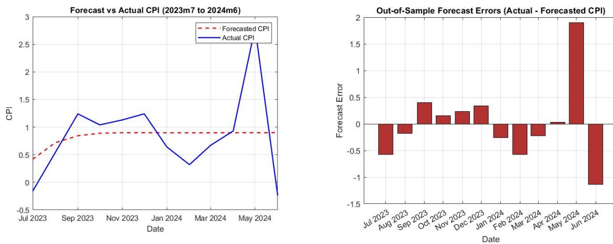
Graph 17. FAVAR with lag 2
