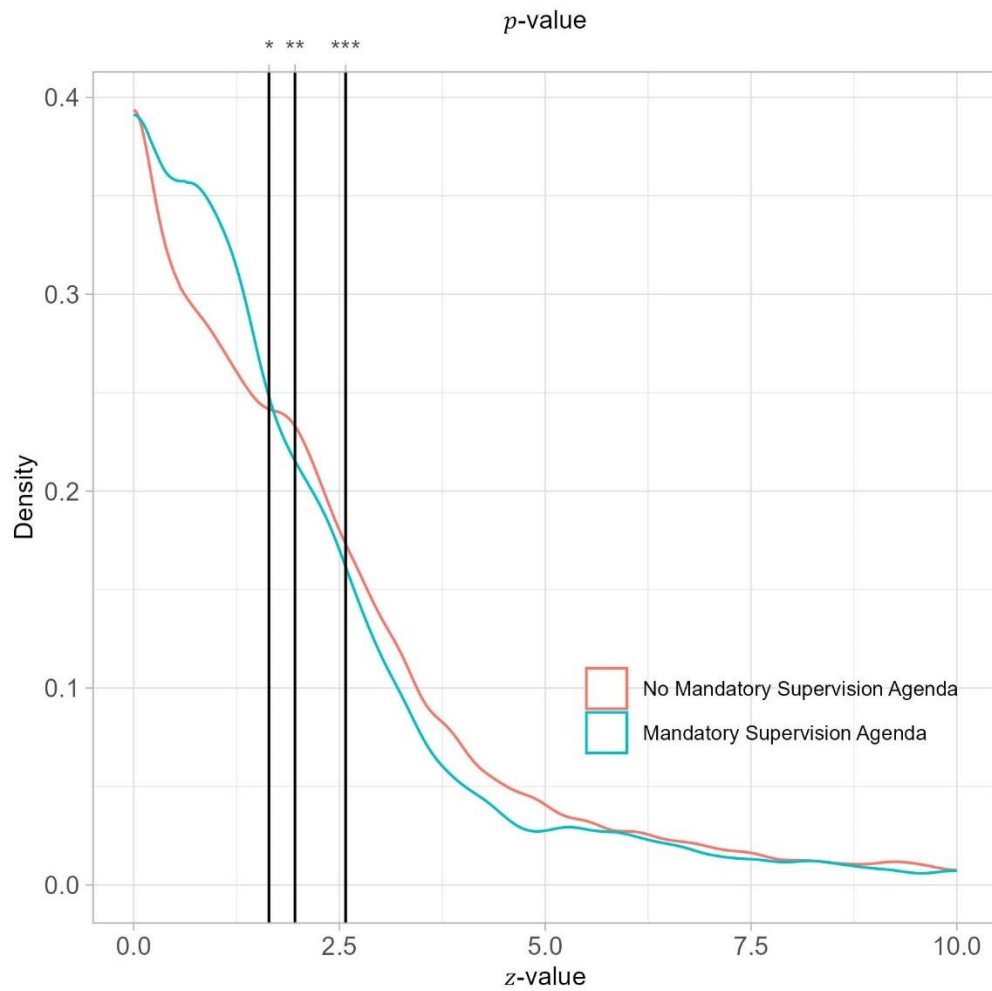
Figure A3. Gaussian density lines of z -values of test statistics from follow-up papers of dissertations and the dissertations themselves considering the presence/absence of mandatory supervision agendas during time of PhD completion and considering only z \in [0, 10] . Black vertical lines depict z -values corresponding to the conventional significance thresholds for 10 percent, 5 percent, and 1 percent. Imprecisely reported z -values removed following (Kranz and Pütz 2022).
