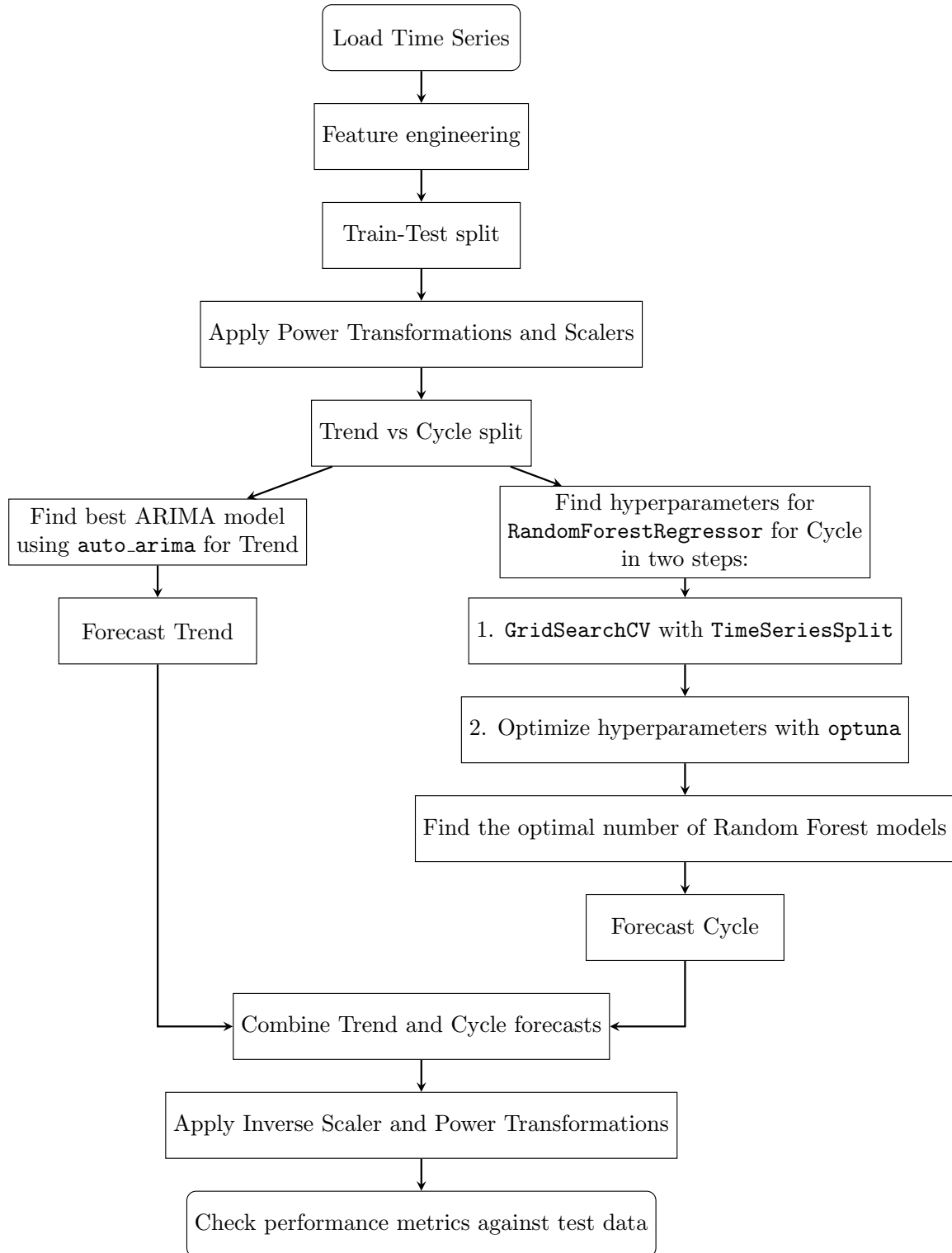
Figure 21: Flowchart of the Forecasting Process with Random Forest
