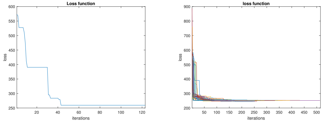
Figure B.28: Loss function in Equation (14) shown for scenario K3m2_1pf. The left panel shows a single optimization with iterative pairwise axis (Givens) rotations. The right panel shows the same for 50 optimizations, using different randomly chosen starting points.
