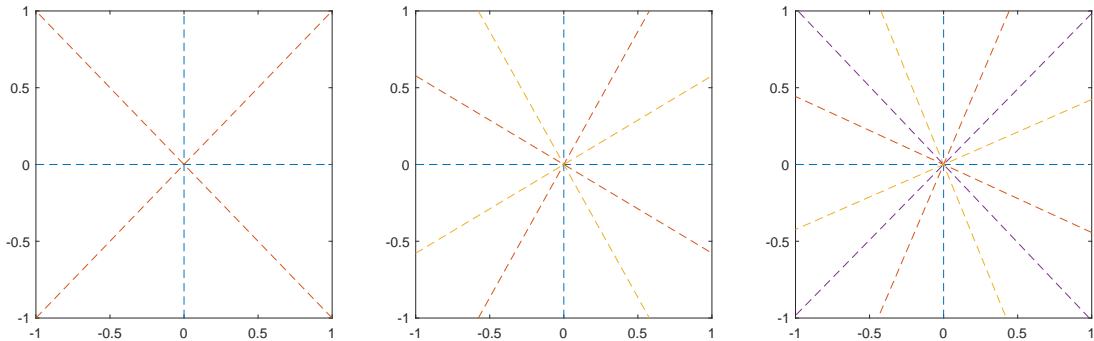
Figure C.31: Minimal correlation solutions for 2, 3 and 4 modes in the 2-dimensional case.
