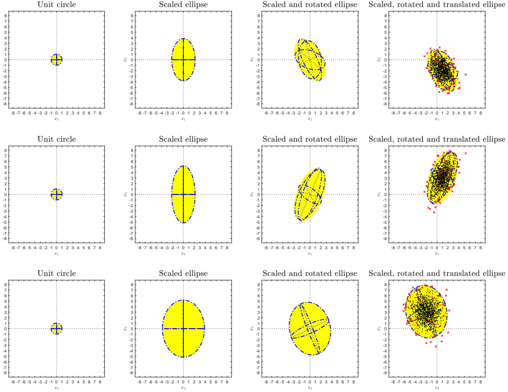
Figure B.27: 95% highest posterior density ellipsoid for K = 3 , built by first expanding the unit ball, then applying a rotation and a translation. Top row shows axes 1 and 2, middle row axes 1 and 3, and bottom row axes 2 and 3. Original data points shown in black (inside the ellipsoid) and red (outside the ellipsoid) in the panels in the right column.
