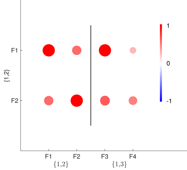
Figure 18: US CPI, sparse permutation. Factor correlations, across factor combinations.
