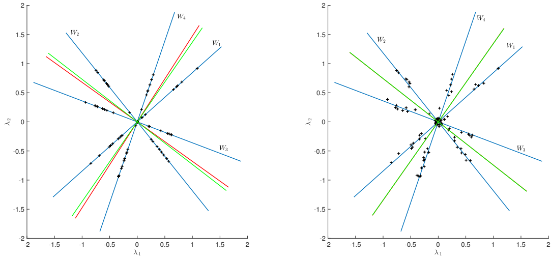
Figure 2: Two exact sparse representations (left) and two “noisy” sparse representations (right) in a two-factor model. Rotation based on the Varimax criterion and based on least square minimization.
