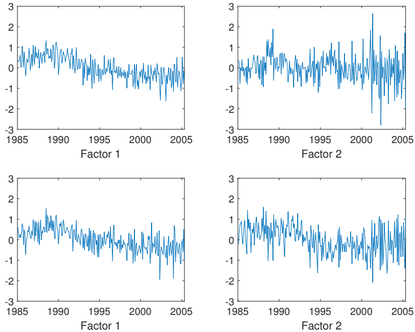
Figure 16: US CPI, unconstrained rotation. Mean factors of Mode 1 (first line) and Mode 2 (second line).
