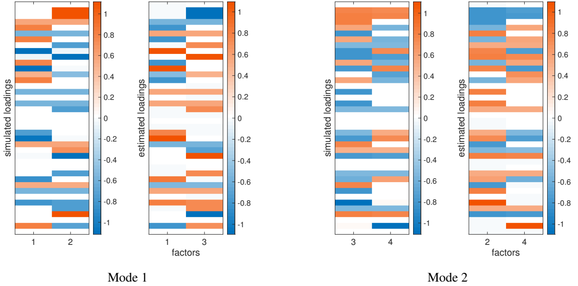
Figure 11: K = 2 , sparse permutation, scenario data50ex_thur_ln. Heat plot of posterior median factor loadings.
