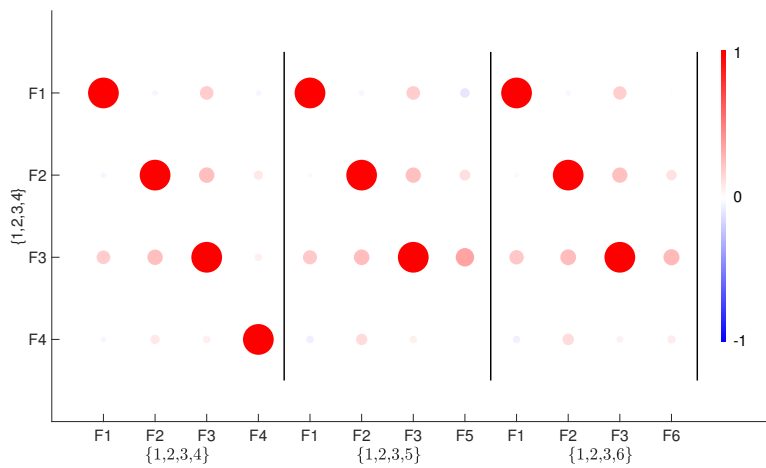
Figure 23: GDP growth, sparse permutation. Factor correlations, across factor combinations.
