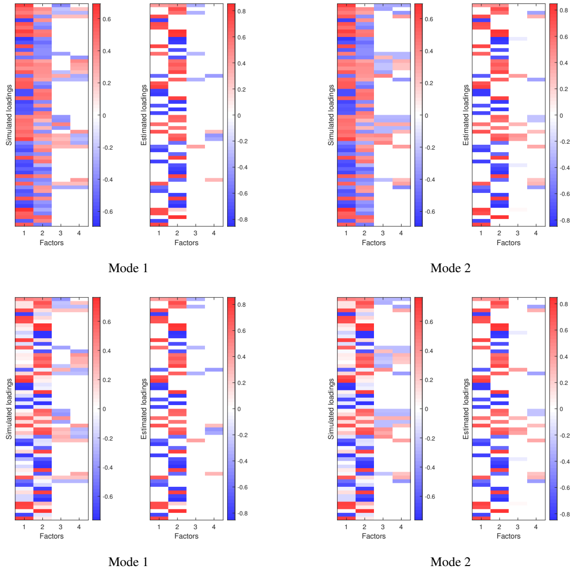
Figure 13: K = 4 , unconstrained rotation, scenario K4m2_2pf. Heat plot of posterior mean factor loadings. Second line: Varimax rotation of simulated loadings for the two pervasive factors.
