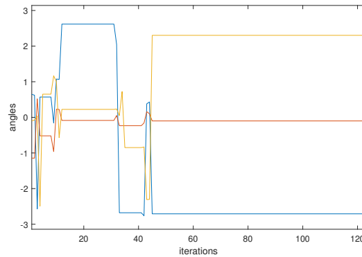
Figure B.29: Givens rotation angles implied by the optimal H_* for the pairwise axis rotations for scenario K3m2_1pf. The blue, red and yellow lines, respectively, denote the angles between axis pairs 1 and 2, 1 and 3, and 2 and 3.
