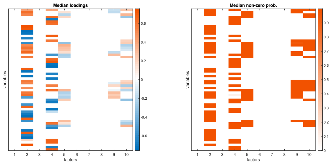
Figure D.34: K = 5 , sparse permutation, scenario K4m2_2pf. Clustered output for overfitted estimate. Factor-specific median factor loadings. Evaluated for factor-specific draws across factor combinations displayed in Table D.8.
