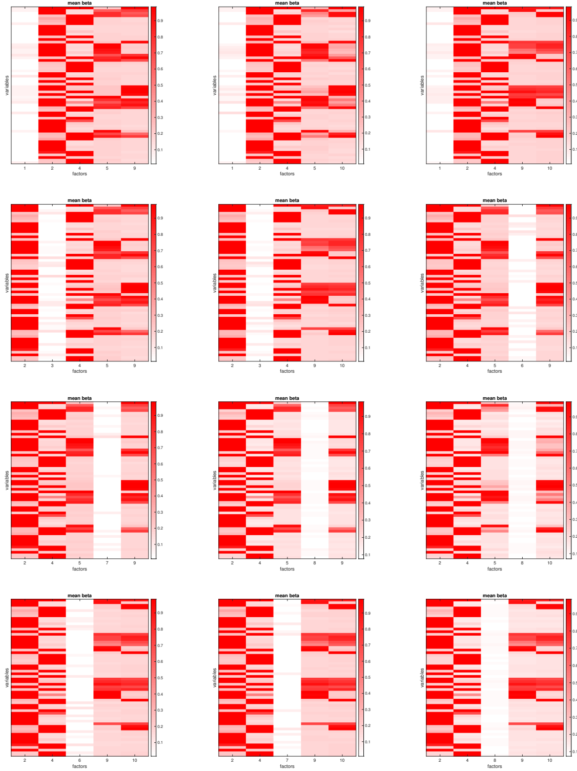
Figure D.36: K = 5 , sparse permutation, scenario K4m2_2pf. Sorted output for overfitted estimate. Mean non-zero probability. See Table D.8 for the number of draws sorted into each factor combination.
