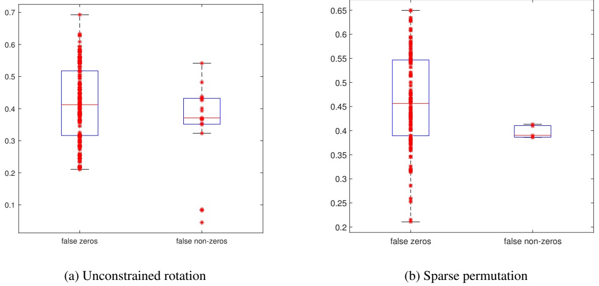
Figure 12: Scenario K4m2_2pf and K4m2_2pf_ln, pooling over modes. Boxplot of absolute factor loadings. The centerline is the median, the edges correspond to the 25th and 75th percentiles (IQR), while the whiskers extend 1.5 times IQR beyond the edges.
