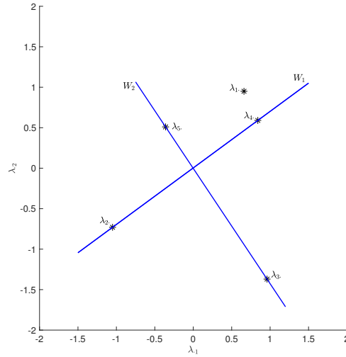
Figure 1: Five factor loadings, four of which are located in 1-dimensional subspaces.
