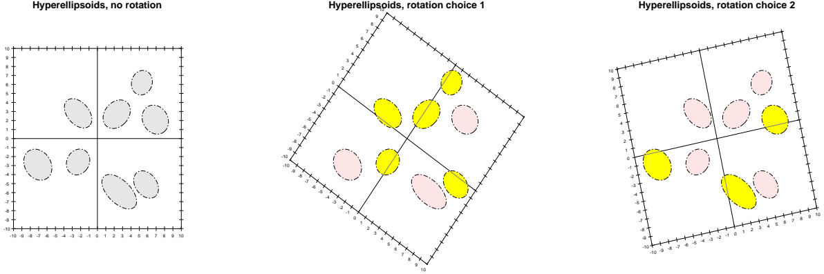
Figure 4: 95% highest posterior density ellipsoids for eight row vectors \lambda_i with K = 2 (first panel), first proposed axis rotation (second panel), and second proposed axis rotation (third panel).
