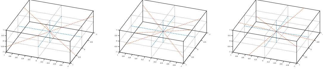
Figure C.32: Three different minimal correlation solutions for 2 modes in the 3-dimensional case.
