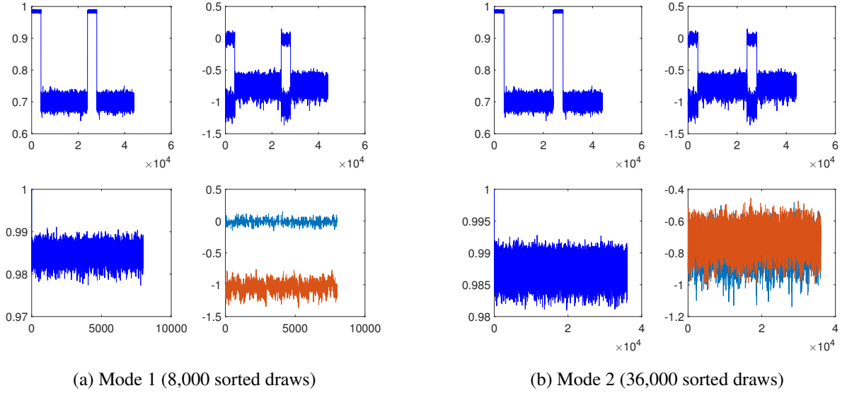
Figure 9: K = 2 , sparse permutation, scenario data50ex_thur_ln. Posterior draws, unsorted and sorted. From top left to bottom right: Correlation of the first with all other posterior draws of factor 1, posterior draws of a selected row of \Lambda , correlation of the first with all other sorted posterior draws of mode-specific factor 1, sorted posterior draws of a mode-specific row of \Lambda .
