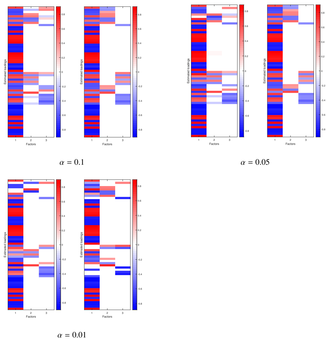
Figure B.30: Results for scenario K3m2_1pf for different choices of \alpha , showing two modes for each choice of \alpha .
