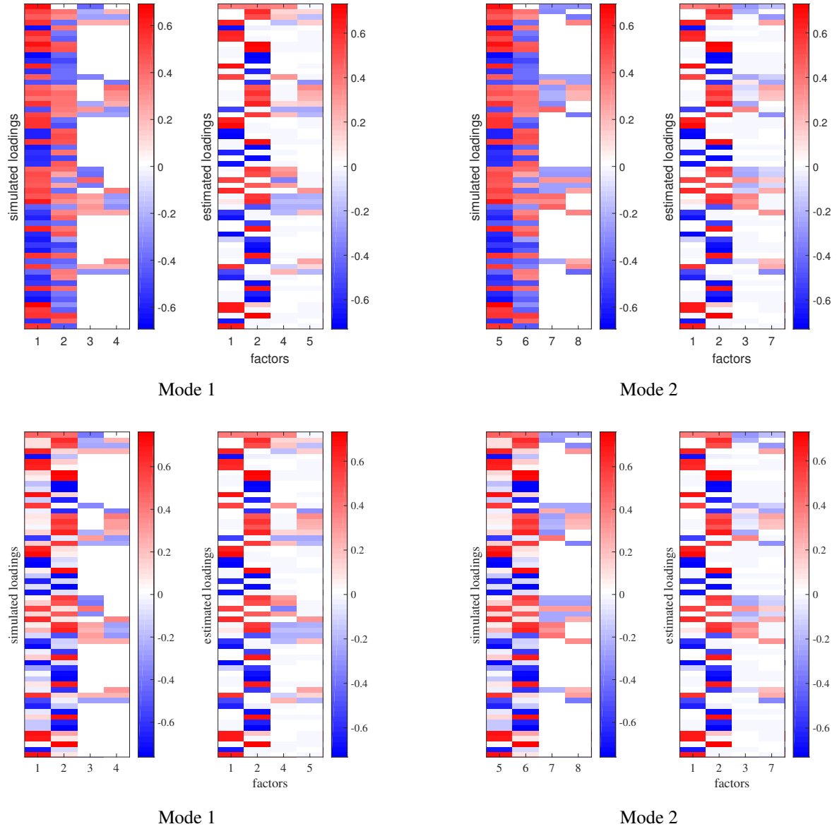
Figure 14: K = 4 , sparse permutation, scenario K4m2_2pf. Heat plot of posterior median factor loadings. Second line: Varimax rotation of simulated loadings of the two pervasive factors.
