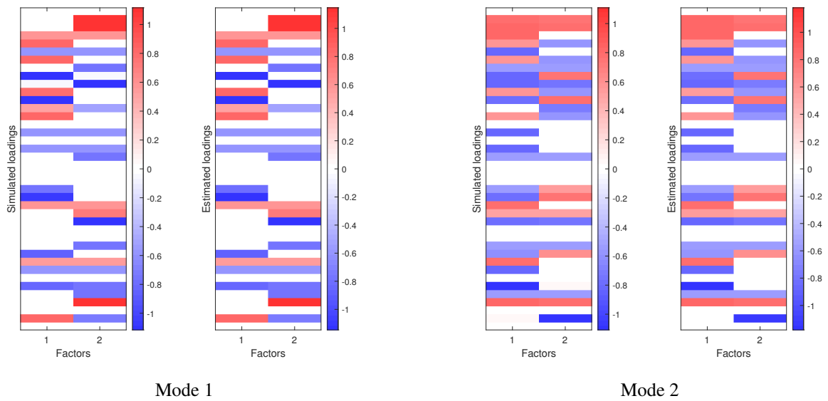
Figure 8: K = 2 , unconstrained rotation, scenario data50ex_thur_ln . Heat plot of posterior mean factor loadings.
